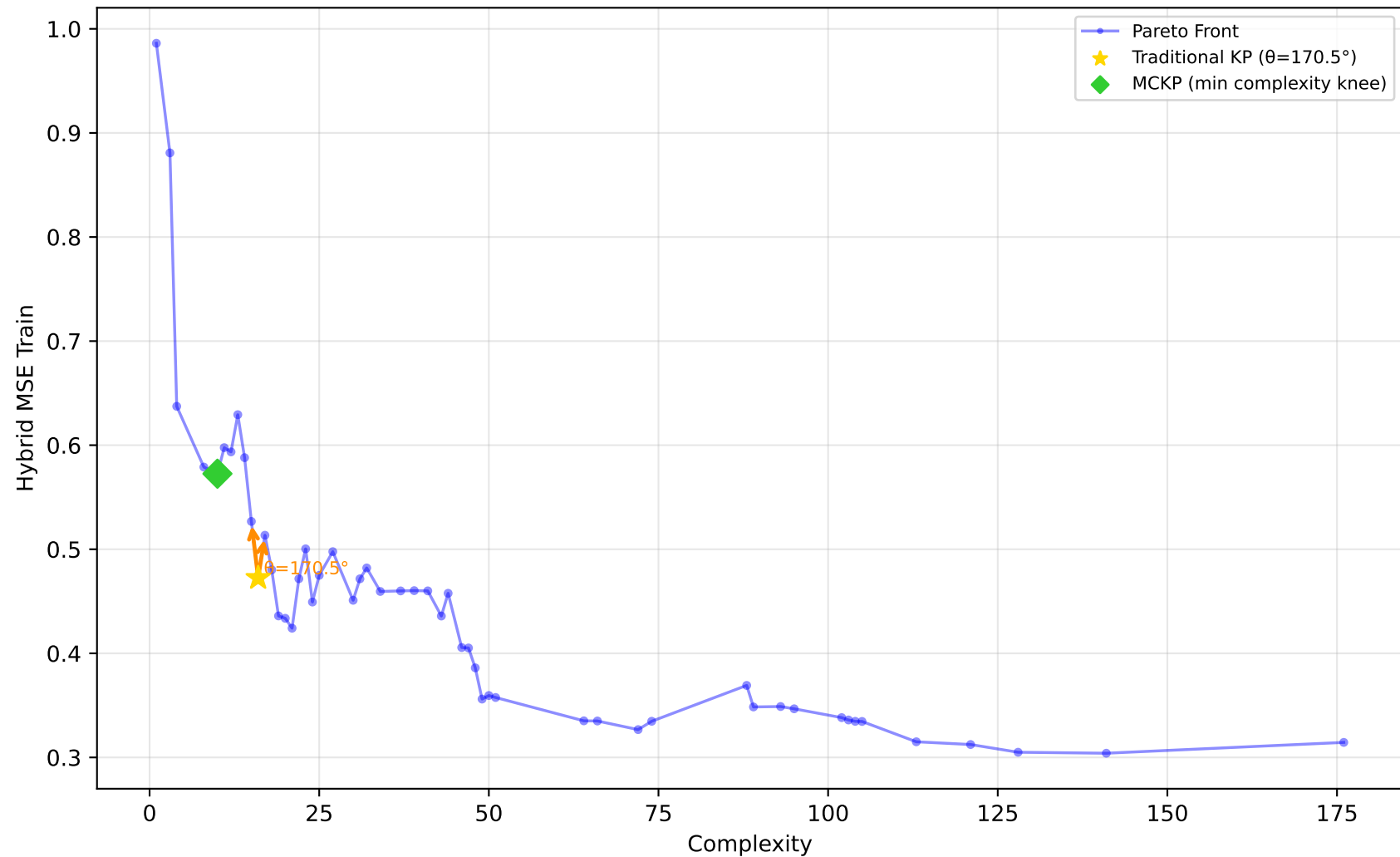
637_fri_c1_500_50 - Run 12 - SVP - Hybrid MSE Train \lambda_1=0.10, \lambda_2=0.00, \lambda_3=0.20 | Difficulty: 1.00 | Method: hmr
