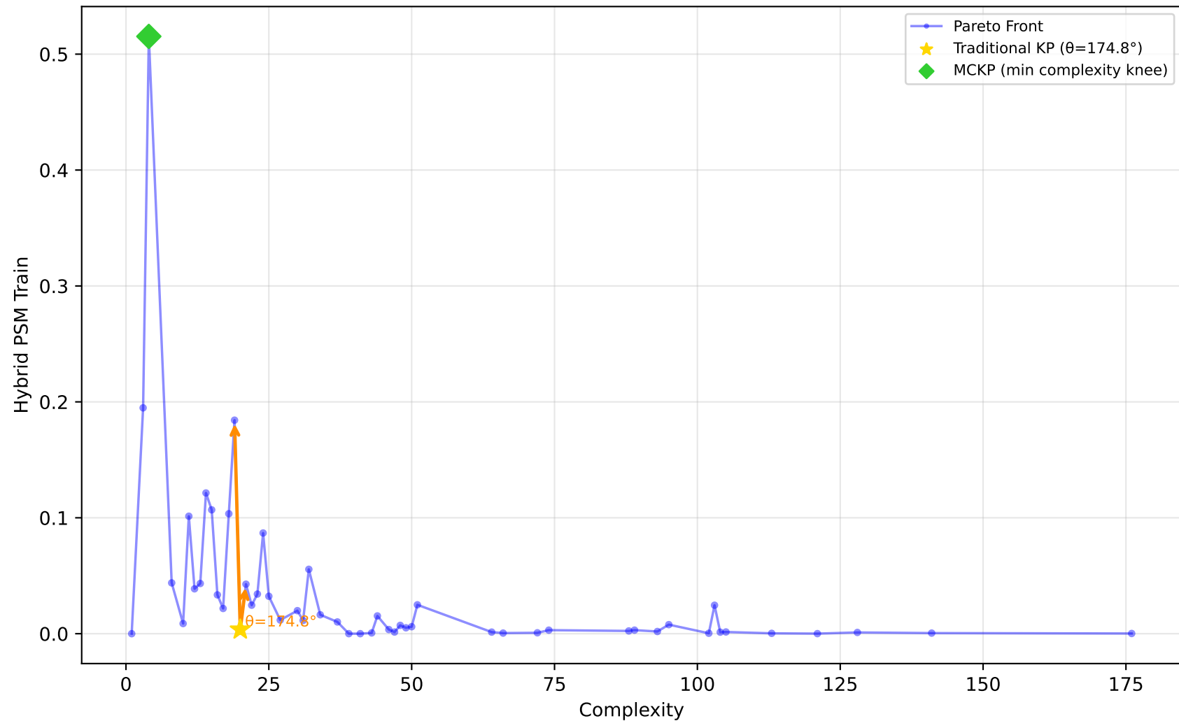
637_fri_c1_500_50 - Run 12 - SVP - Hybrid PSM Train \lambda_1=0.00, \lambda_2=0.00, \lambda_3=0.00 | Difficulty: 1.00 | Method: hmr
