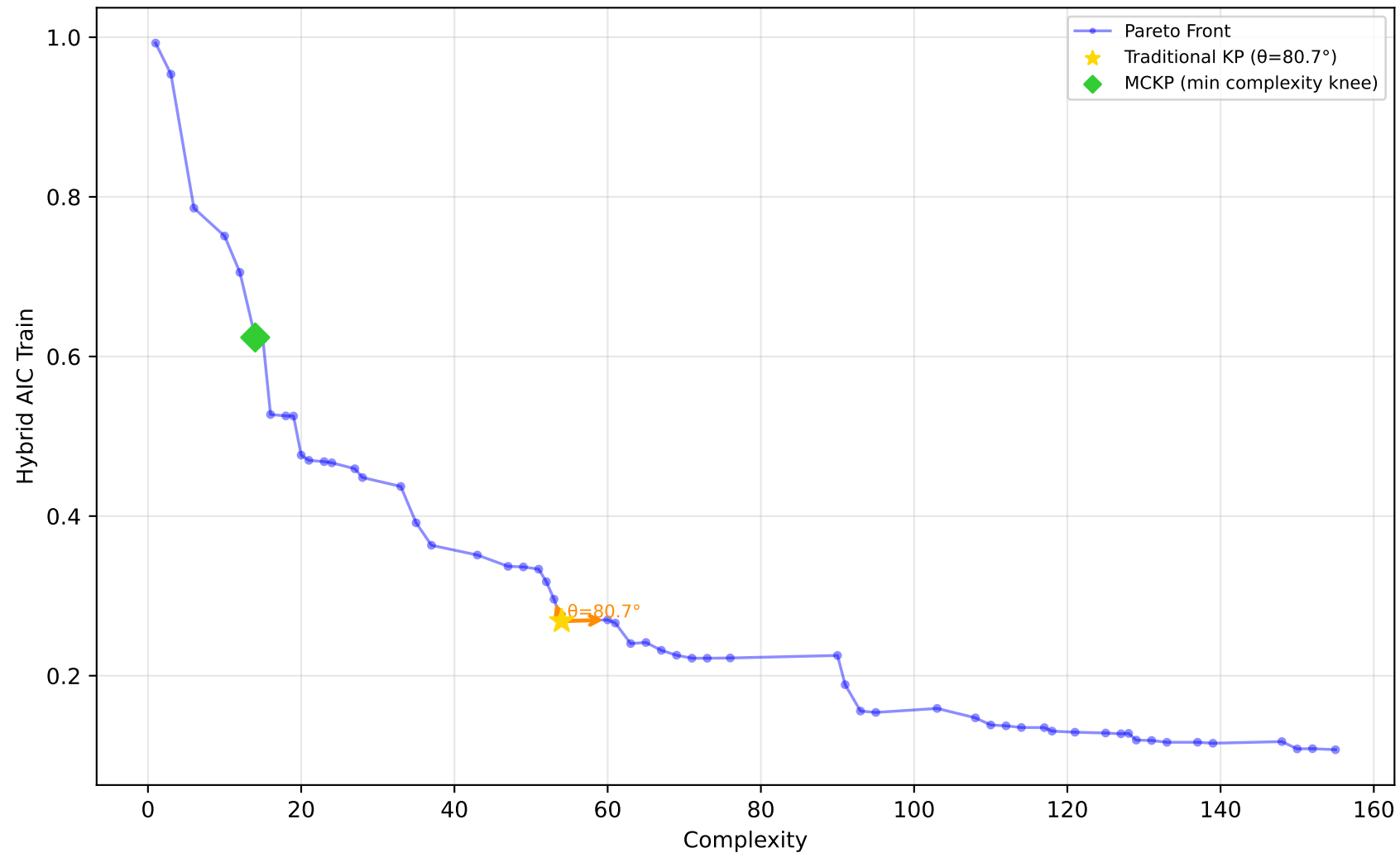
637_fri_c1_500_50 - Run 13 - MVP - Hybrid AIC Train \lambda_1=0.00, \lambda_2=0.50, \lambda_3=0.00 | Difficulty: 1.00 | Method: hmr
