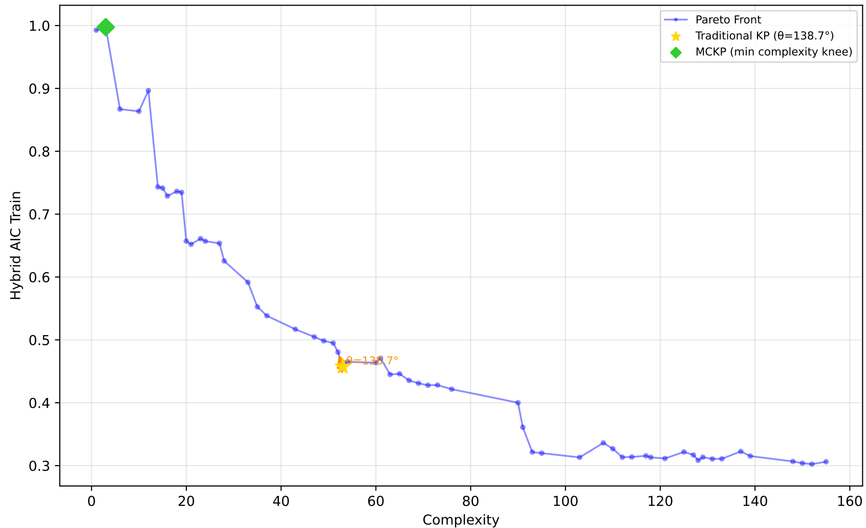
637_fri_c1_500_50 - Run 13 - MVP - Hybrid AIC Train \lambda_1=0.10, \lambda_2=0.00, \lambda_3=1.00 | Difficulty: 1.00 | Method: hmr
