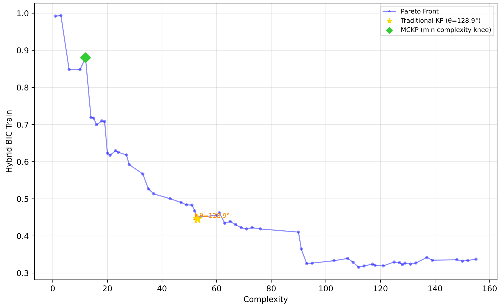
637_fri_c1_500_50 - Run 13 - MVP - Hybrid BIC Train \lambda_1=0.10, \lambda_2=0.00, \lambda_3=1.00 | Difficulty: 1.00 | Method: hmr
