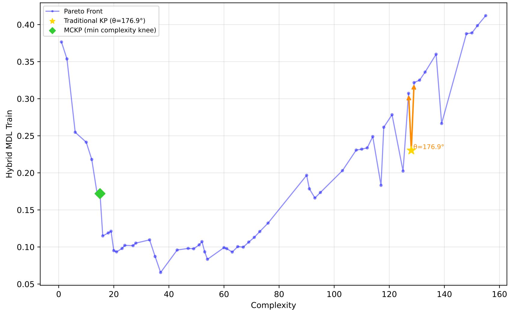
637_fri_c1_500_50 - Run 13 - MVP - Hybrid MDL Train \lambda_1=0.00, \bar{\lambda}_2=0.50, \lambda_3=0.00 | Difficulty: 1.00 | Method: hmr
