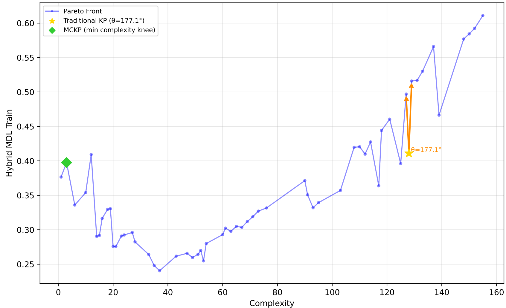
637_fri_c1_500_50 - Run 13 - MVP - Hybrid MDL Train \lambda_1=0.10, \lambda_2=0.00, \lambda_3=1.00 | Difficulty: 1.00 | Method: hmr
