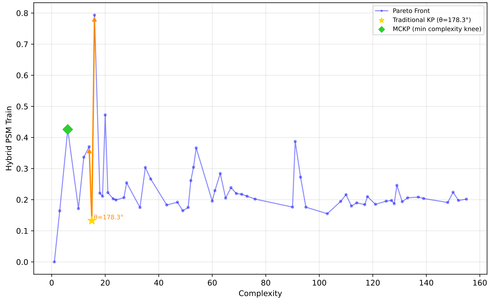
637_fri_c1_500_50 - Run 13 - MVP - Hybrid PSM Train \lambda_1=0.10, \bar{\lambda}_2=0.00, \bar{\lambda}_3=1.00 | Difficulty: 1.00 | Method: hmr
