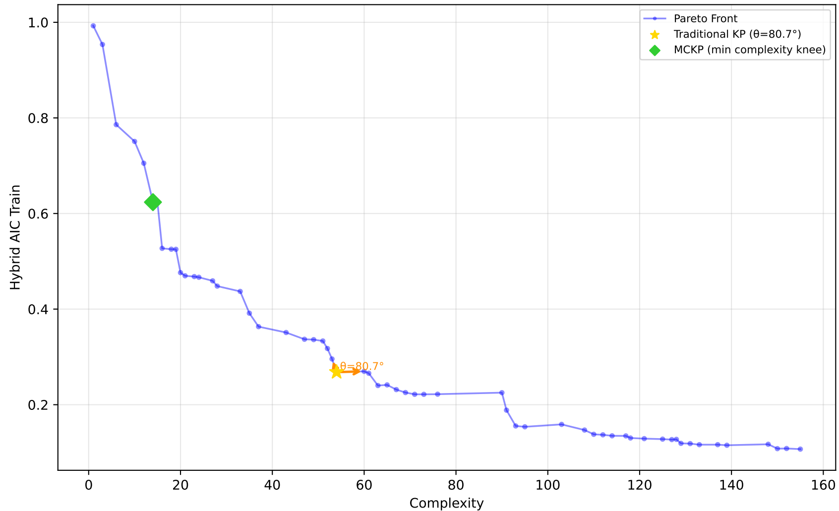
637_fri_c1_500_50 - Run 13 - SVP - Hybrid AIC Train \lambda_1=0.00, \lambda_2=0.00, \lambda_3=0.00 | Difficulty: 1.00 | Method: hmr
