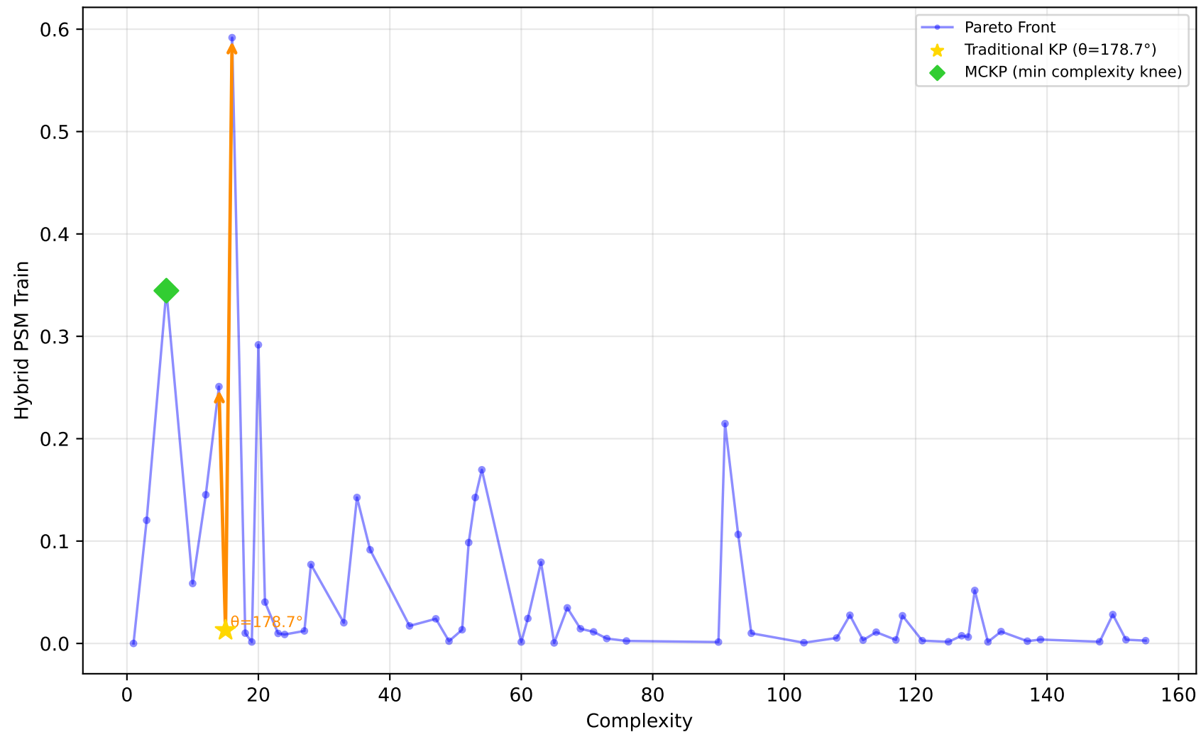
637_fri_c1_500_50 - Run 13 - SVP - Hybrid PSM Train \lambda_1=0.00, \lambda_2=0.00, \lambda_3=0.00 | Difficulty: 1.00 | Method: hmr
