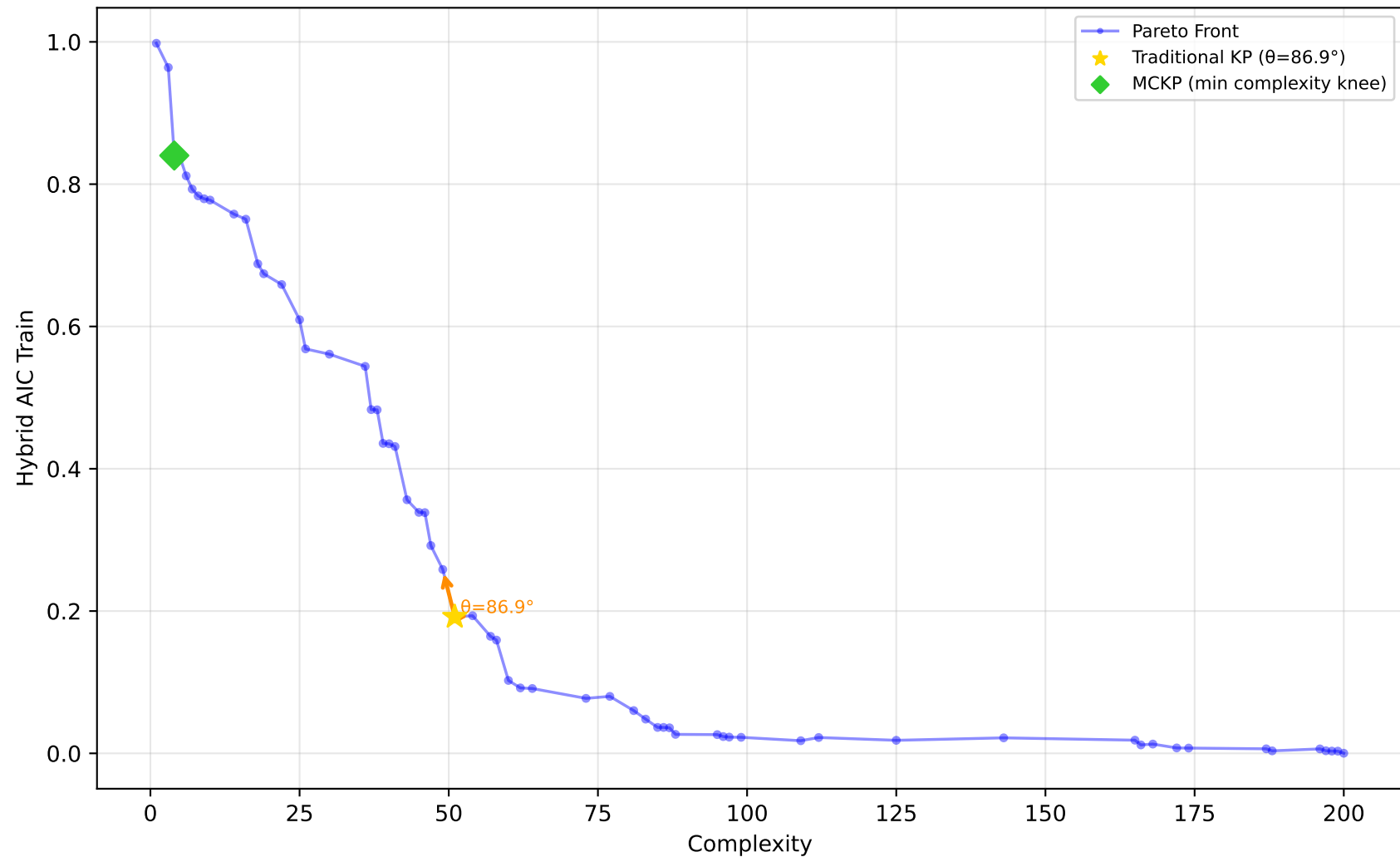
637_fri_c1_500_50 - Run 14 - MVP - Hybrid AIC Train \lambda_1=0.00, \lambda_2=0.50, \lambda_3=0.00 | Difficulty: 1.00 | Method: hmr
