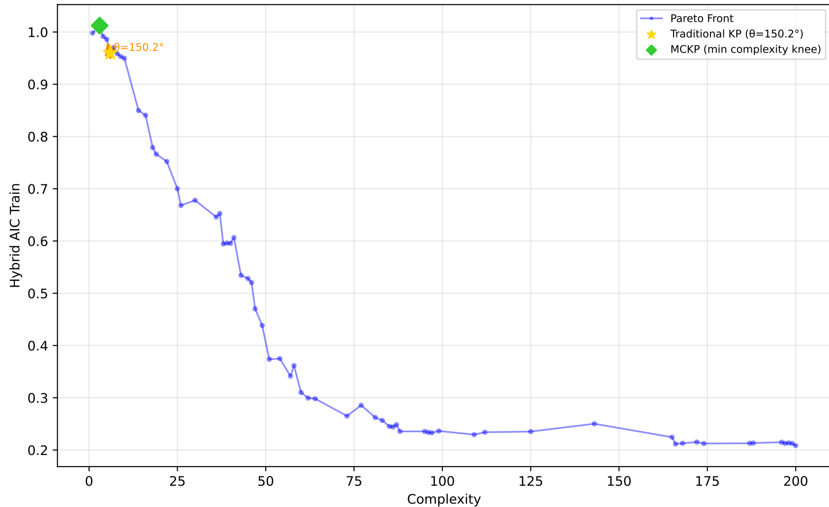
637_fri_c1_500_50 - Run 14 - MVP - Hybrid AIC Train \lambda_1=0.10, \lambda_2=0.00, \lambda_3=1.00 | Difficulty: 1.00 | Method: hmr
