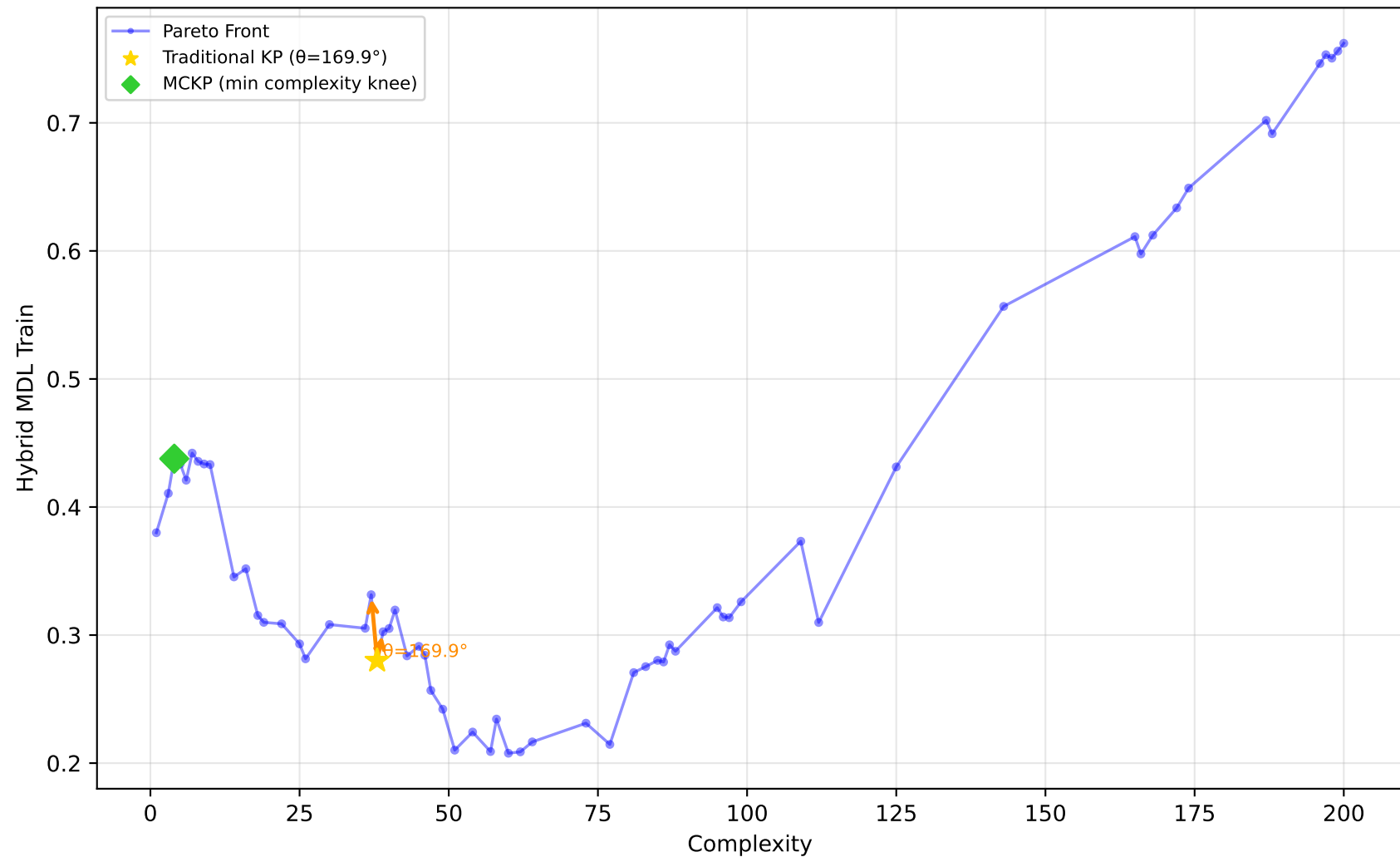
637_fri_c1_500_50 - Run 14 - MVP - Hybrid MDL Train \lambda_1=0.10, \bar{\lambda}_2=0.00, \lambda_3=1.00 | Difficulty: 1.00 | Method: hmr
