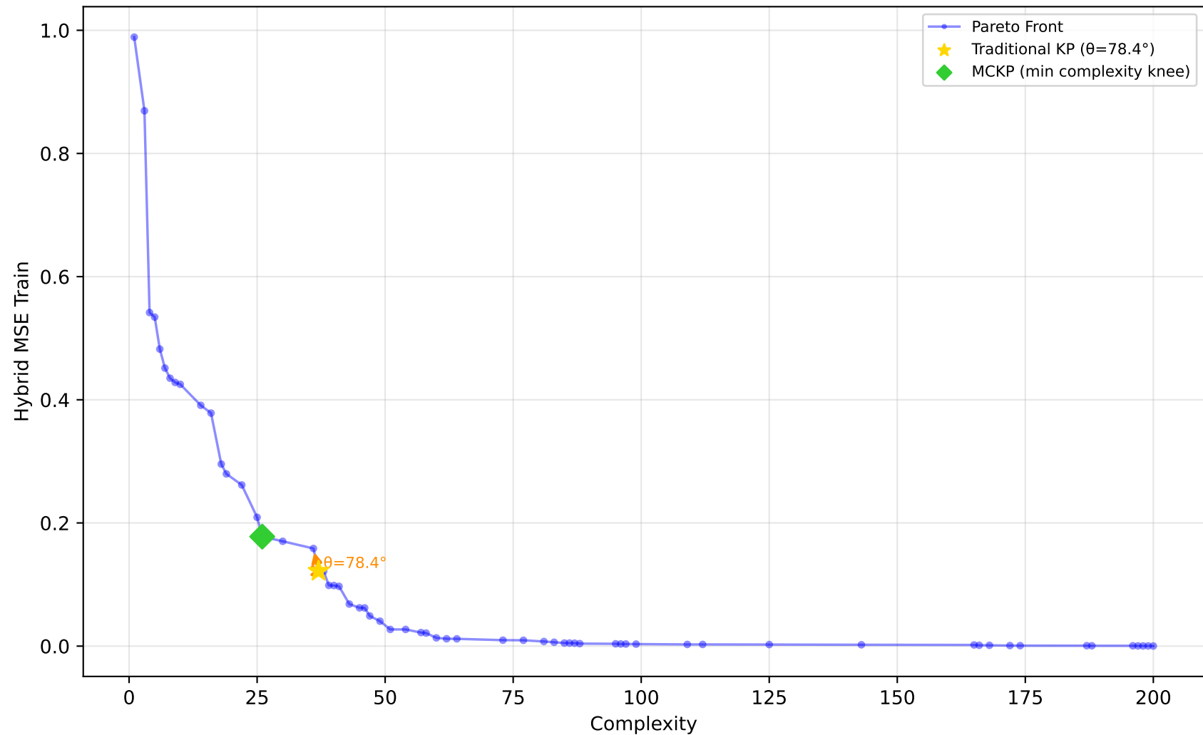
637_fri_c1_500_50 - Run 14 - MVP - Hybrid MSE Train \lambda_1=0.00, \bar{\lambda}_2=0.50, \lambda_3=0.00 | Difficulty: 1.00 | Method: hmr
