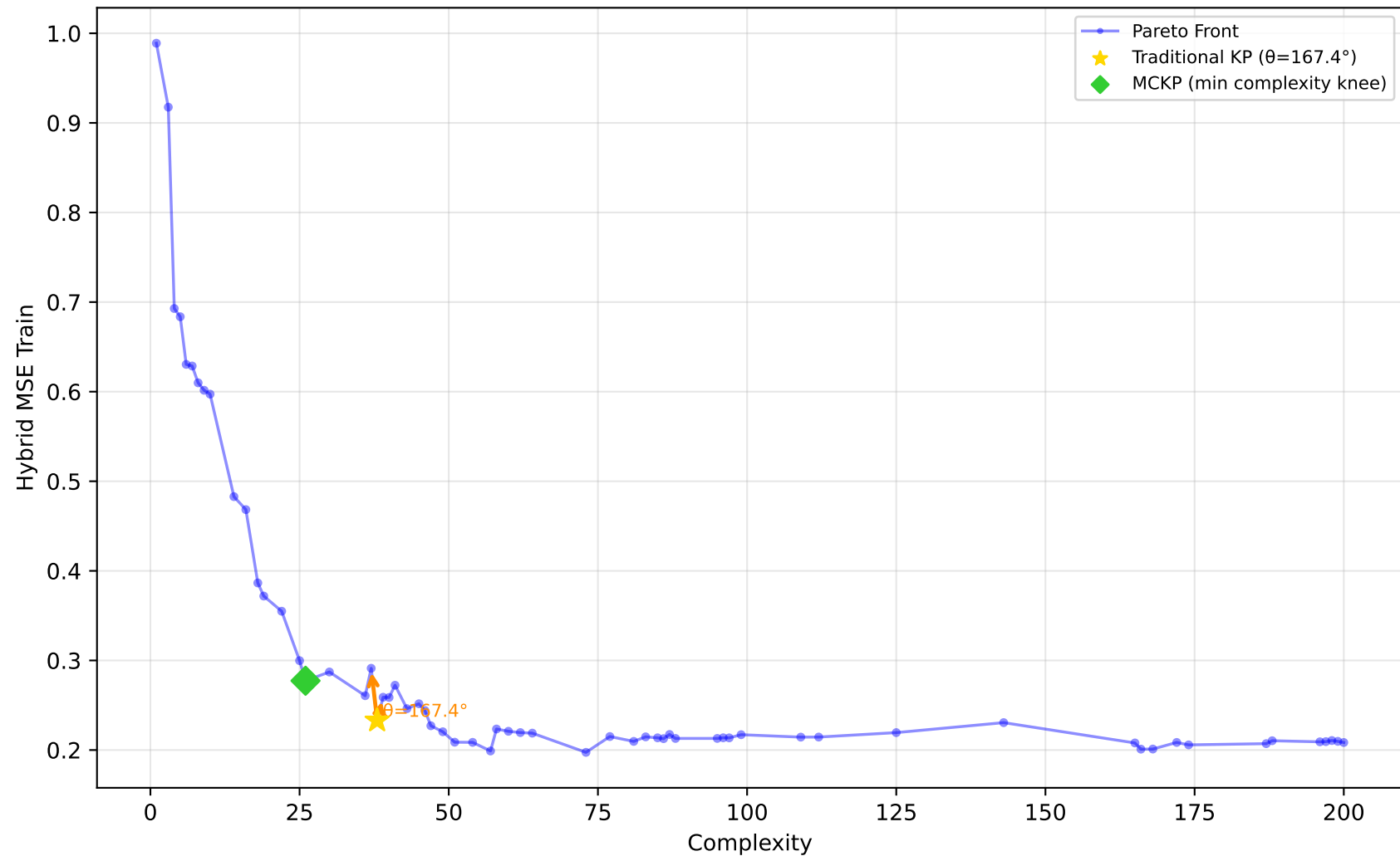
637_fri_c1_500_50 - Run 14 - MVP - Hybrid MSE Train \lambda_1=0.10, \bar{\lambda}_2=0.00, \bar{\lambda}_3=1.00 | Difficulty: 1.00 | Method: hmr
