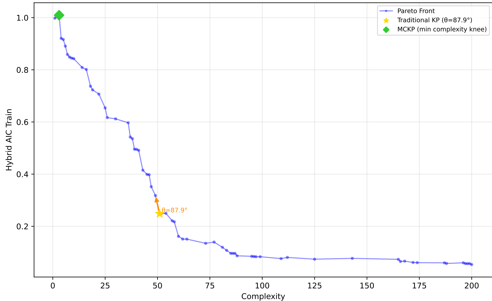
637_fri_c1_500_50 - Run 14 - SVP - Hybrid AIC Train \lambda_1=0.10, \lambda_2=0.00, \lambda_3=0.20 | Difficulty: 1.00 | Method: hmr
