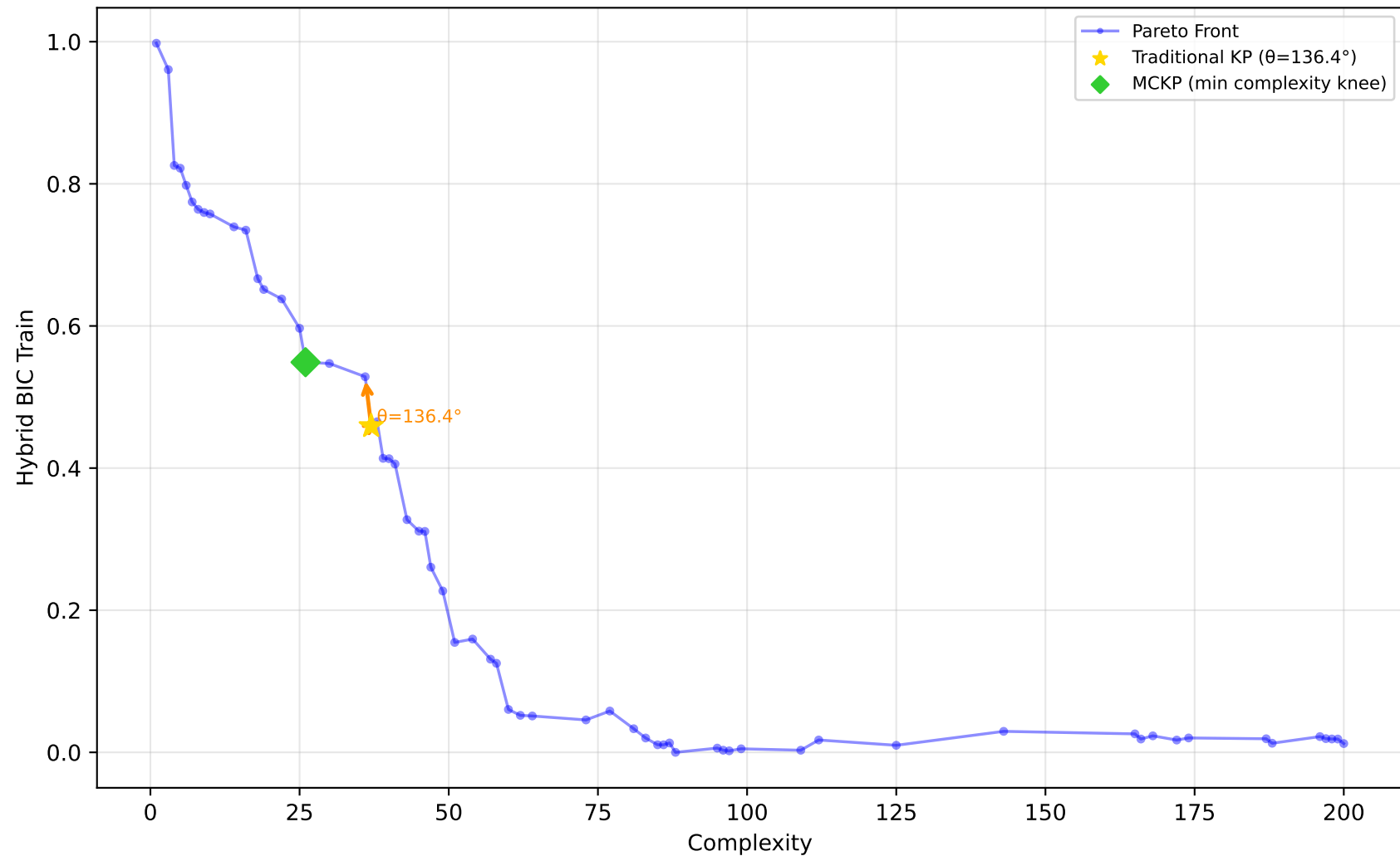
637_fri_c1_500_50 - Run 14 - SVP - Hybrid BIC Train \lambda_1=0.00, \lambda_2=0.00, \lambda_3=0.00 | Difficulty: 1.00 | Method: hmr
