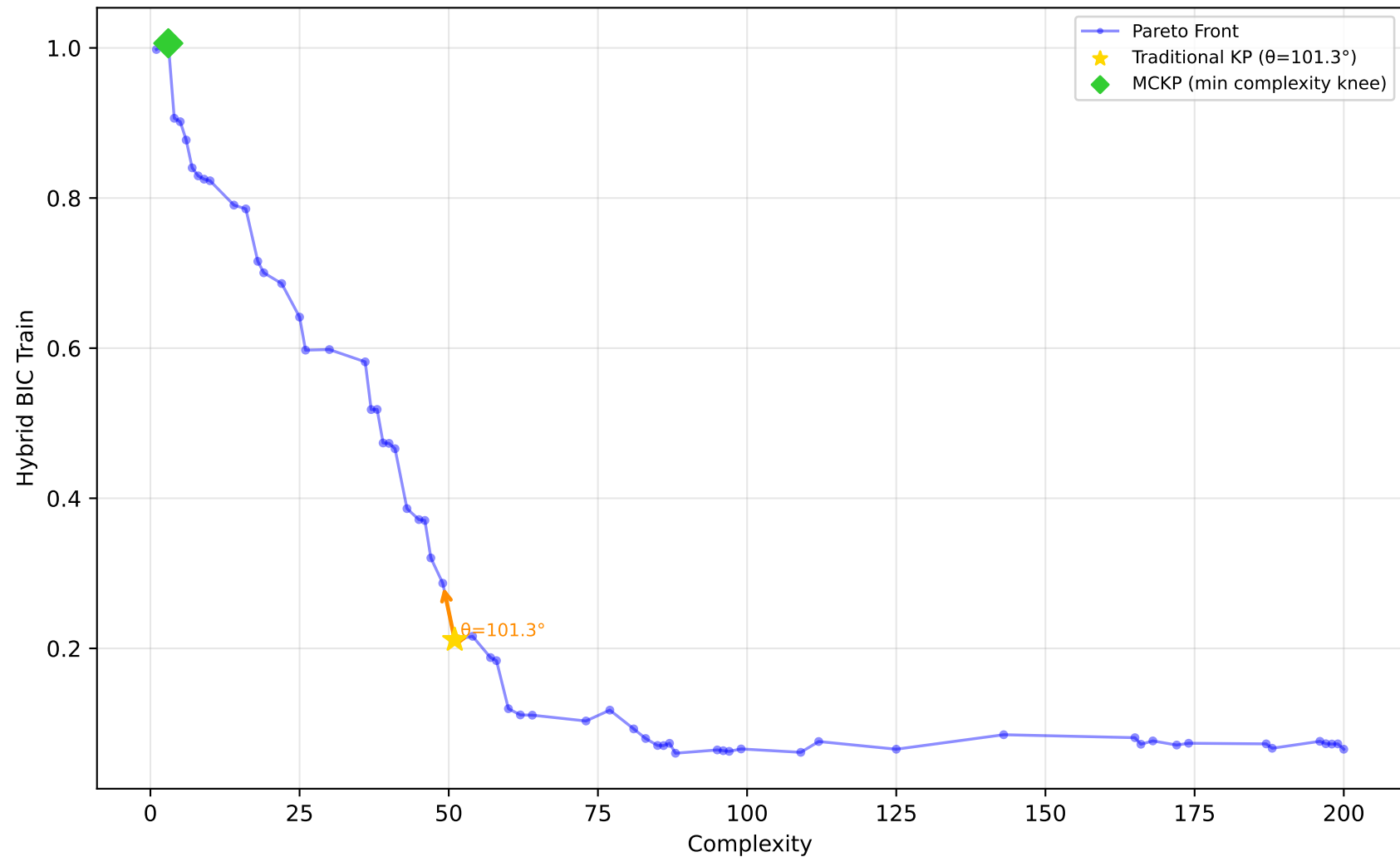
637_fri_c1_500_50 - Run 14 - SVP - Hybrid BIC Train \lambda_1=0.10, \lambda_2=0.00, \lambda_3=0.20 | Difficulty: 1.00 | Method: hmr
