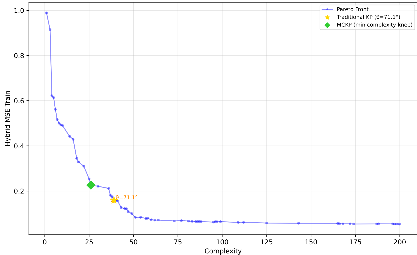
637_fri_c1_500_50 - Run 14 - SVP - Hybrid MSE Train \lambda_1=0.10, \lambda_2=0.00, \lambda_3=0.20 | Difficulty: 1.00 | Method: hmr
