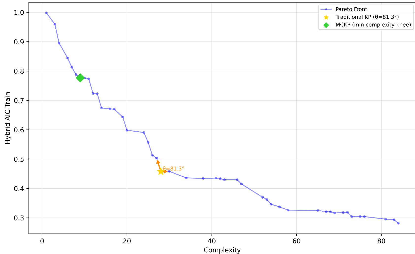
637_fri_c1_500_50 - Run 15 - MVP - Hybrid AIC Train \lambda_1=0.00, \lambda_2=0.50, \lambda_3=0.00 | Difficulty: 1.00 | Method: hmr
