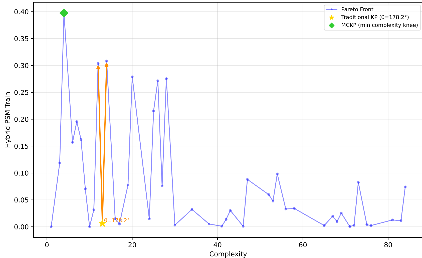
637_fri_c1_500_50 - Run 15 - MVP - Hybrid PSM Train \lambda_1=0.00, \lambda_2=0.50, \lambda_3=0.00 | Difficulty: 1.00 | Method: hmr
