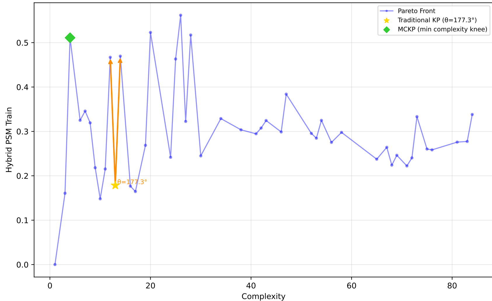
637_fri_c1_500_50 - Run 15 - MVP - Hybrid PSM Train \lambda_1=0.10, \bar{\lambda}_2=0.00, \bar{\lambda}_3=1.00 | Difficulty: 1.00 | Method: hmr
