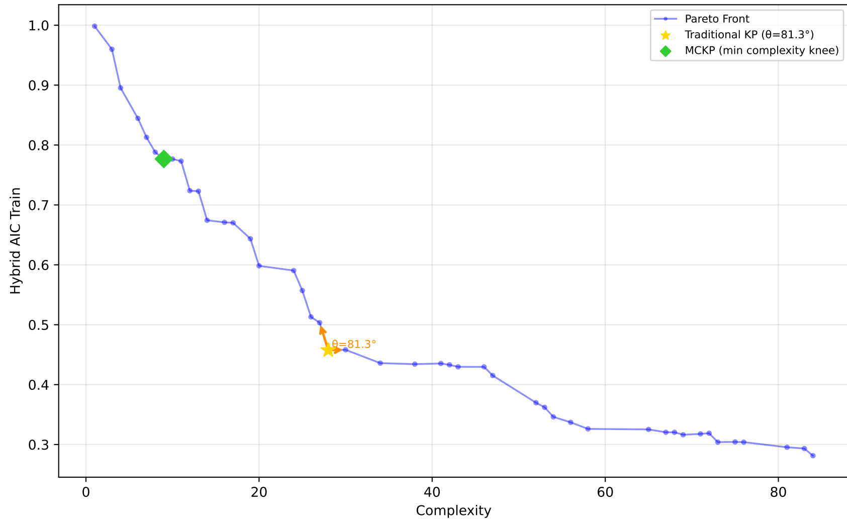
637_fri_c1_500_50 - Run 15 - SVP - Hybrid AIC Train \lambda_1=0.00, \lambda_2=0.00, \lambda_3=0.00 | Difficulty: 1.00 | Method: hmr
