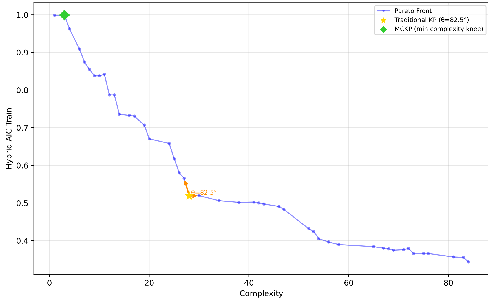
637_fri_c1_500_50 - Run 15 - SVP - Hybrid AIC Train \lambda_1=0.10, \lambda_2=0.00, \lambda_3=0.20 | Difficulty: 1.00 | Method: hmr
