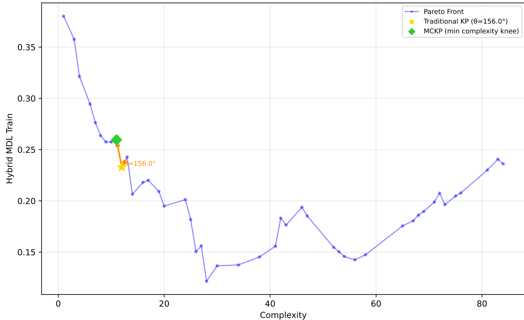
637_fri_c1_500_50 - Run 15 - SVP - Hybrid MDL Train \lambda_1=0.00 , \lambda_2=0.00 , \lambda_3=0.00 | Difficulty: 1.00 | Method: hmr
