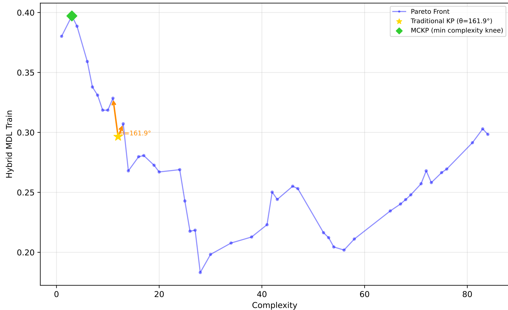
637_fri_c1_500_50 - Run 15 - SVP - Hybrid MDL Train \lambda_1=0.10, \lambda_2=0.00, \lambda_3=0.20 | Difficulty: 1.00 | Method: hmr
