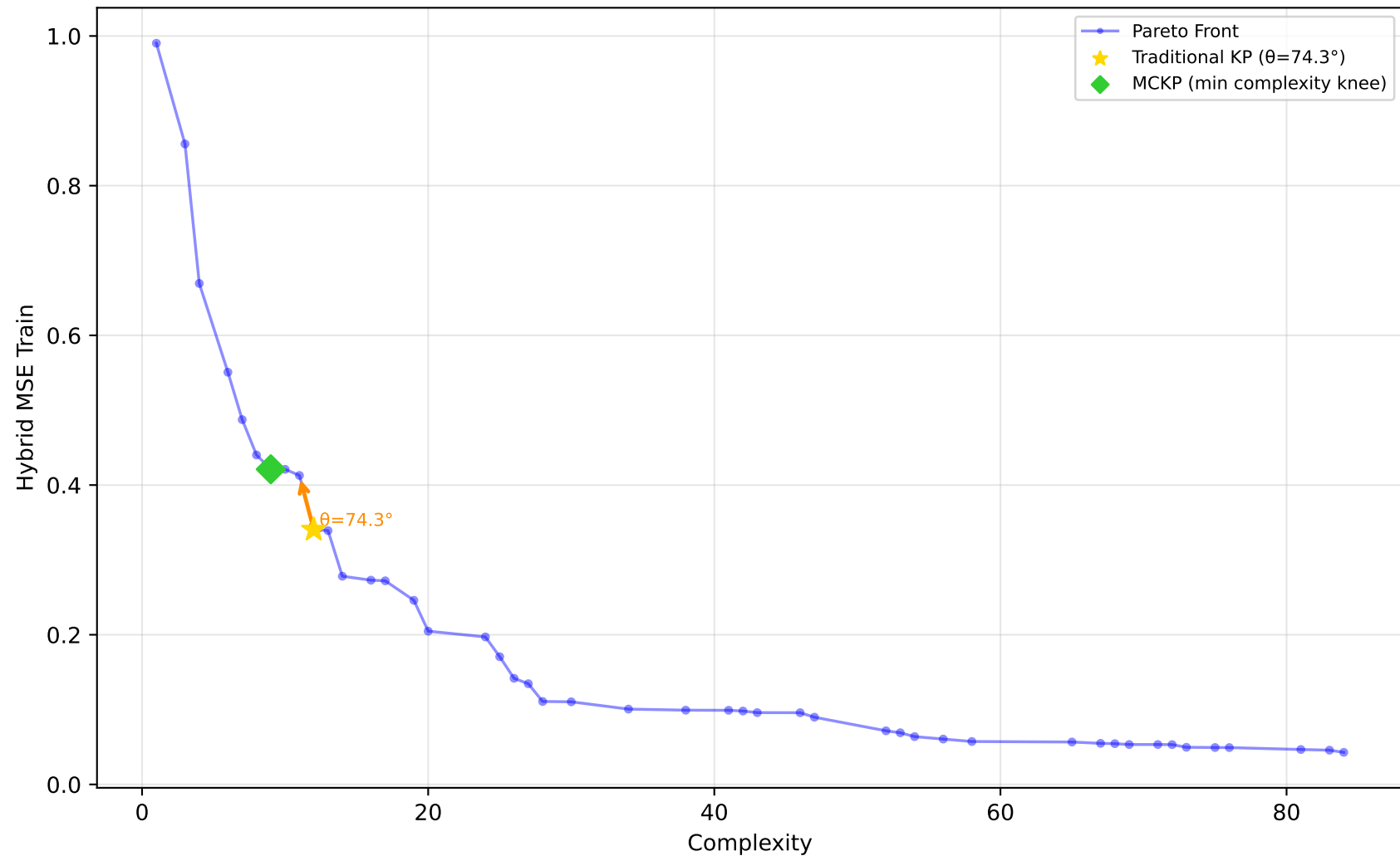
637_fri_c1_500_50 - Run 15 - SVP - Hybrid MSE Train \lambda_1=0.00, \lambda_2=0.00, \lambda_3=0.00 | Difficulty: 1.00 | Method: hmr
