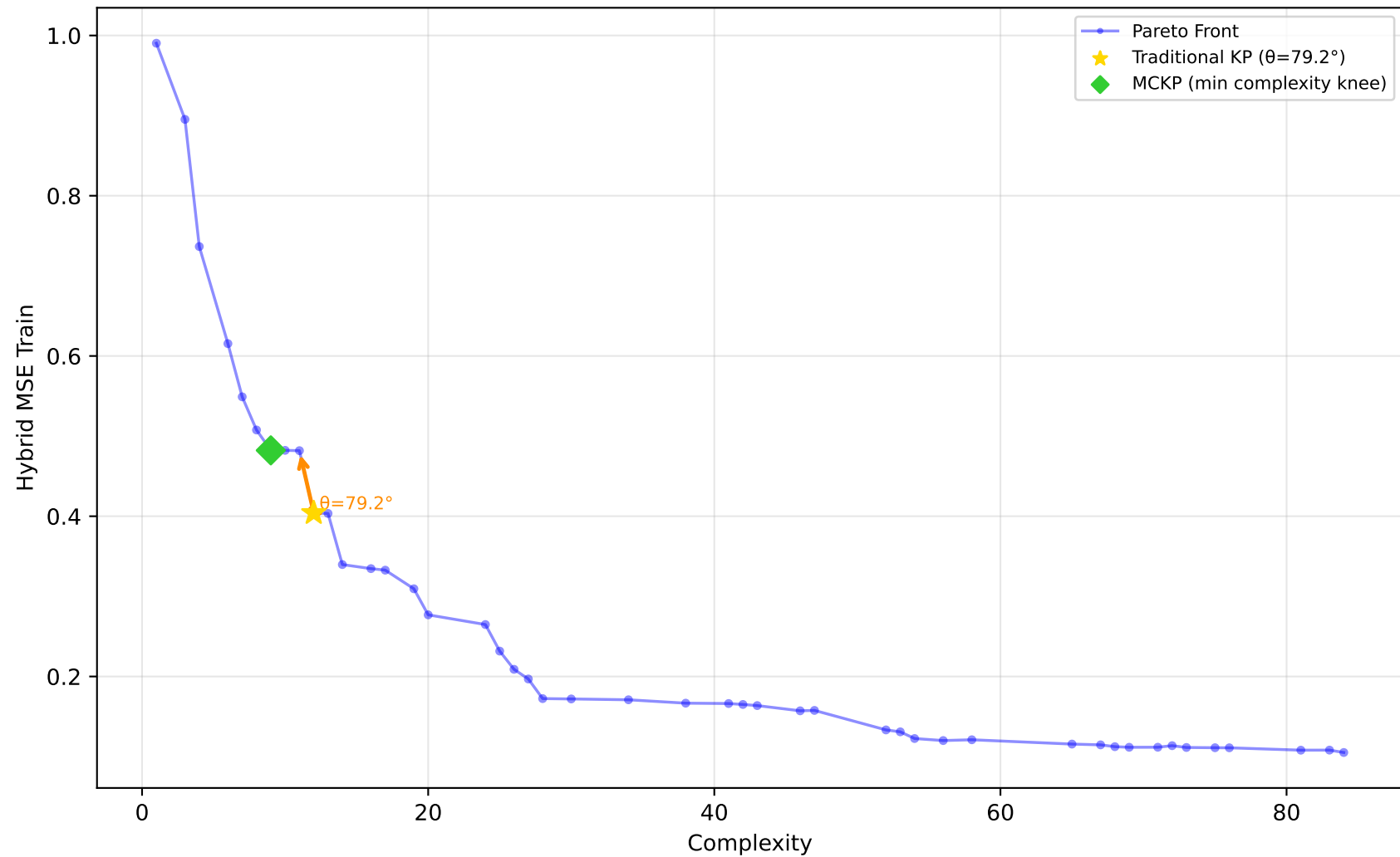
637_fri_c1_500_50 - Run 15 - SVP - Hybrid MSE Train \lambda_1=0.10, \lambda_2=0.00, \lambda_3=0.20 | Difficulty: 1.00 | Method: hmr
