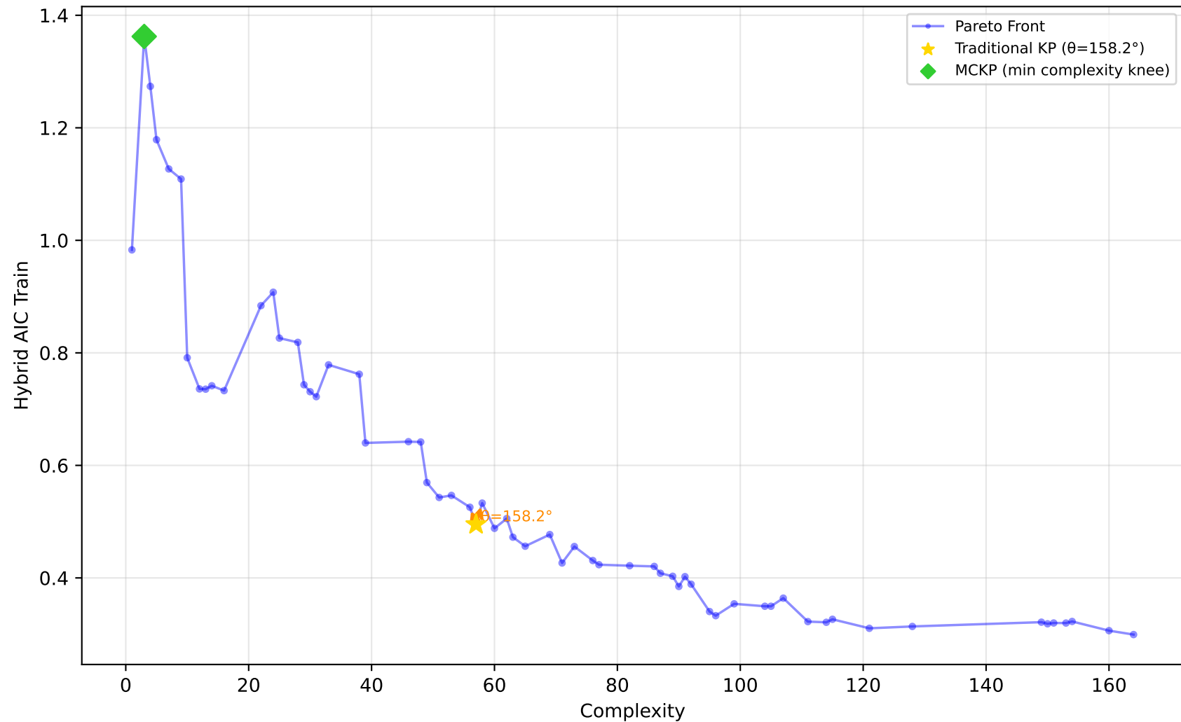
637_fri_c1_500_50 - Run 16 - MVP - Hybrid AIC Train \lambda_1=0.10, \lambda_2=0.00, \lambda_3=1.00 | Difficulty: 1.00 | Method: hmr
