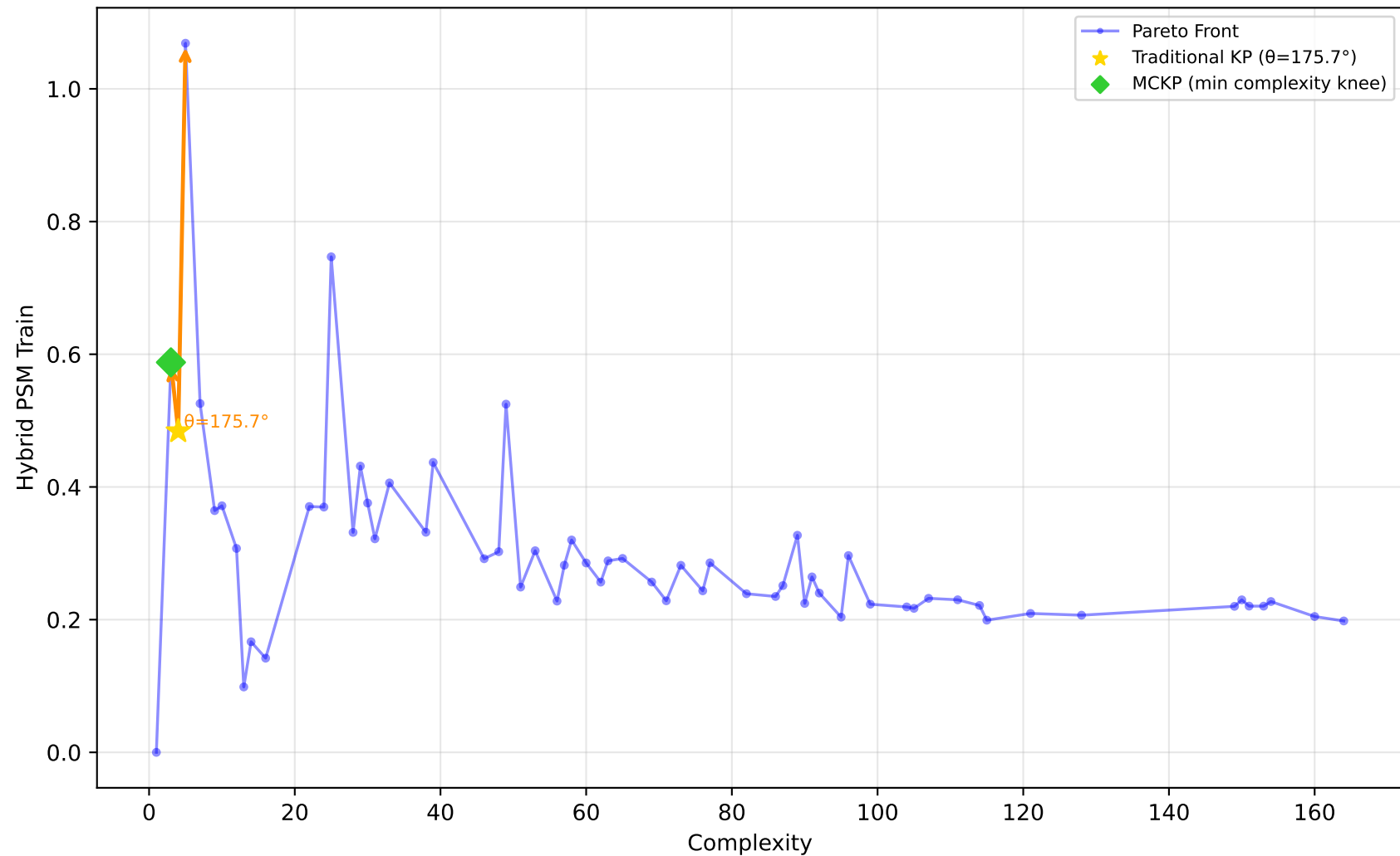
637_fri_c1_500_50 - Run 16 - MVP - Hybrid PSM Train \lambda_1=0.10, \lambda_2=0.00, \lambda_3=1.00 | Difficulty: 1.00 | Method: hmr
