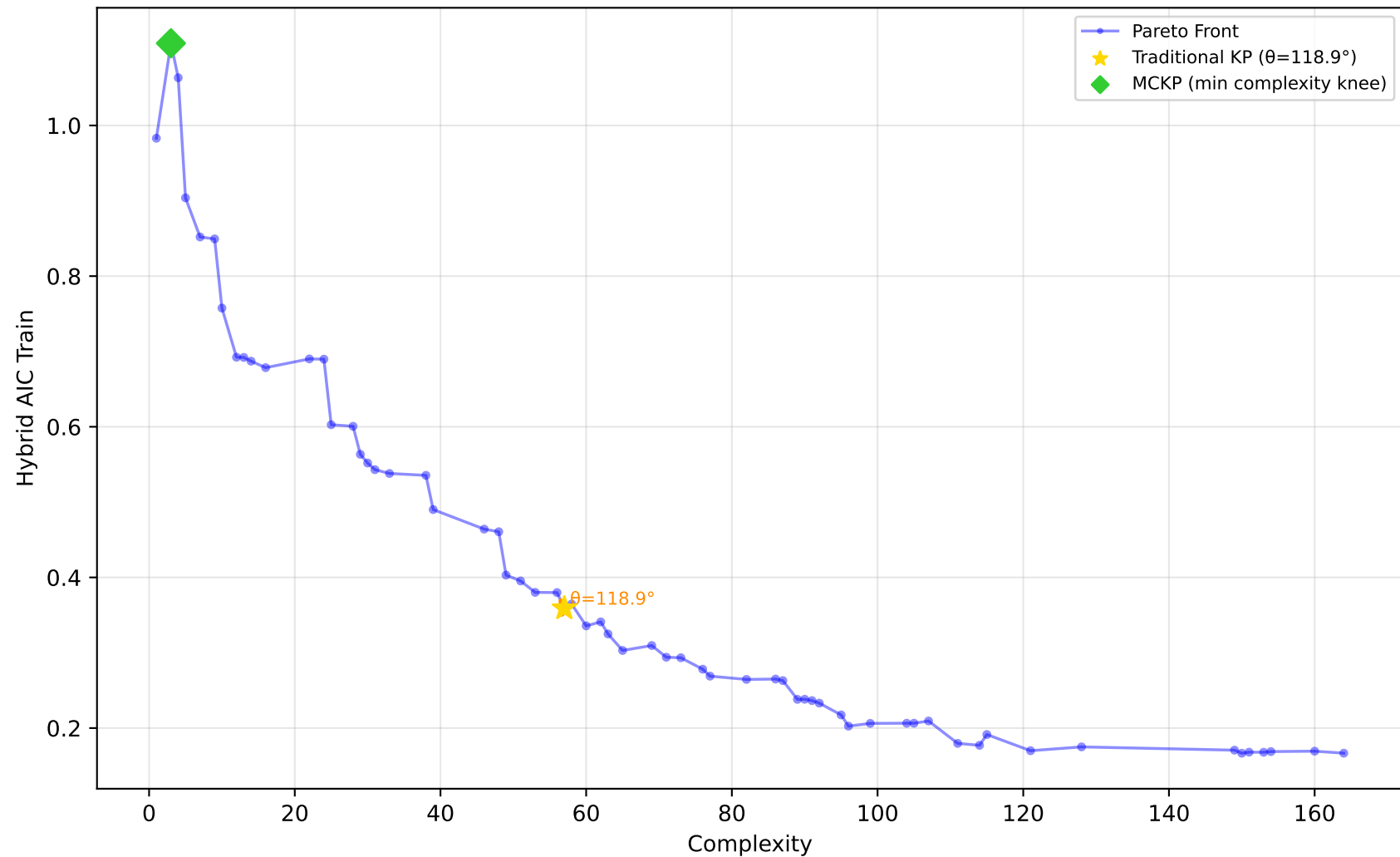
637_fri_c1_500_50 - Run 16 - SVP - Hybrid AIC Train \lambda_1=0.10, \lambda_2=0.00, \lambda_3=0.20 | Difficulty: 1.00 | Method: hmr
