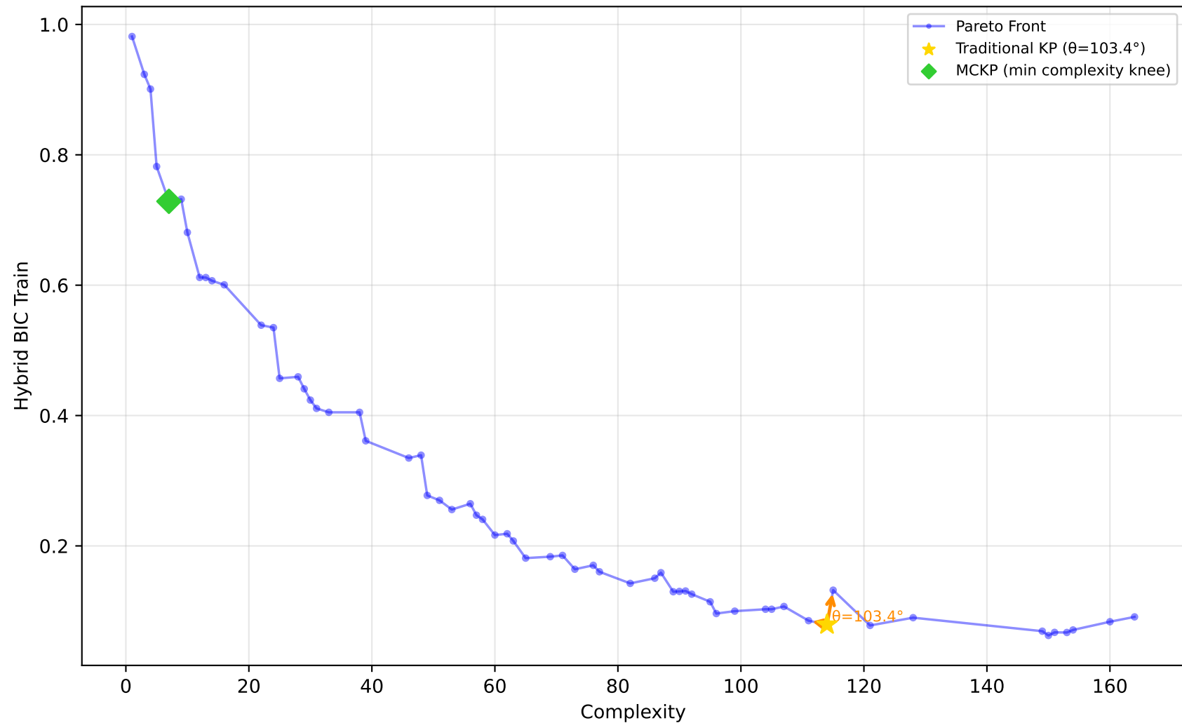
637_fri_c1_500_50 - Run 16 - SVP - Hybrid BIC Train \lambda_1=0.00, \lambda_2=0.00, \lambda_3=0.00 | Difficulty: 1.00 | Method: hmr
