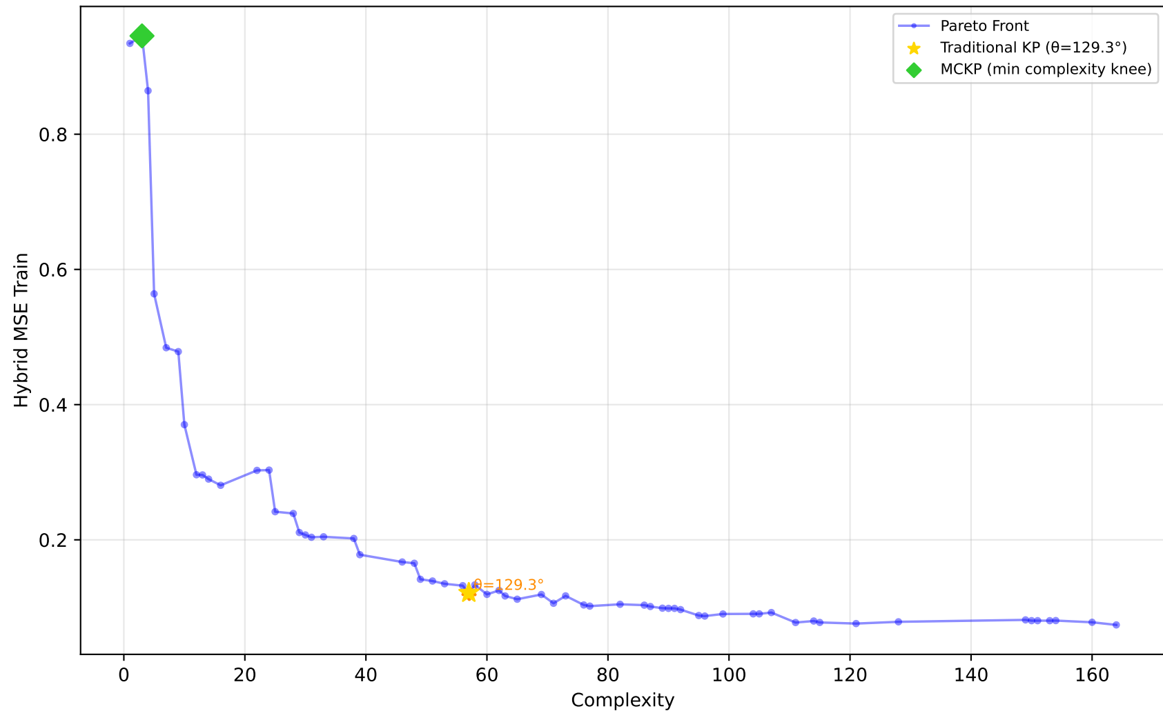
637_fri_c1_500_50 - Run 16 - SVP - Hybrid MSE Train \lambda_1=0.10, \lambda_2=0.00, \lambda_3=0.20 | Difficulty: 1.00 | Method: hmr
