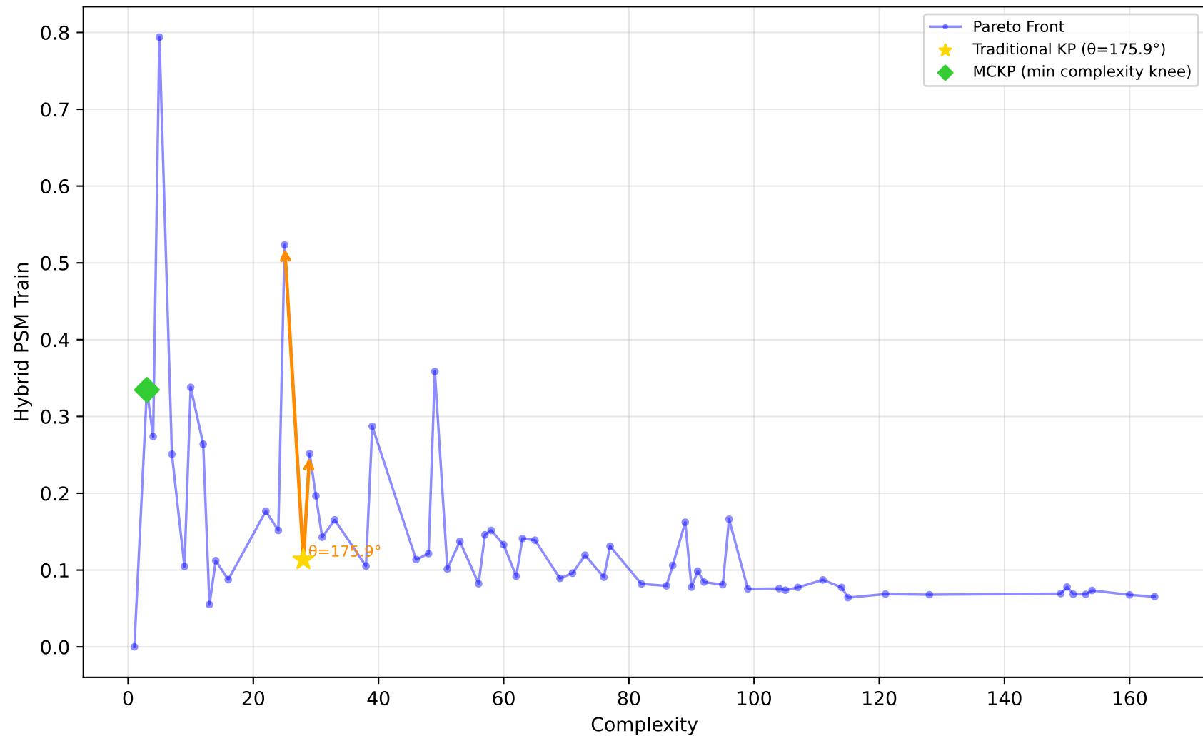
637_fri_c1_500_50 - Run 16 - SVP - Hybrid PSM Train \lambda_1=0.10, \lambda_2=0.00, \lambda_3=0.20 | Difficulty: 1.00 | Method: hmr
