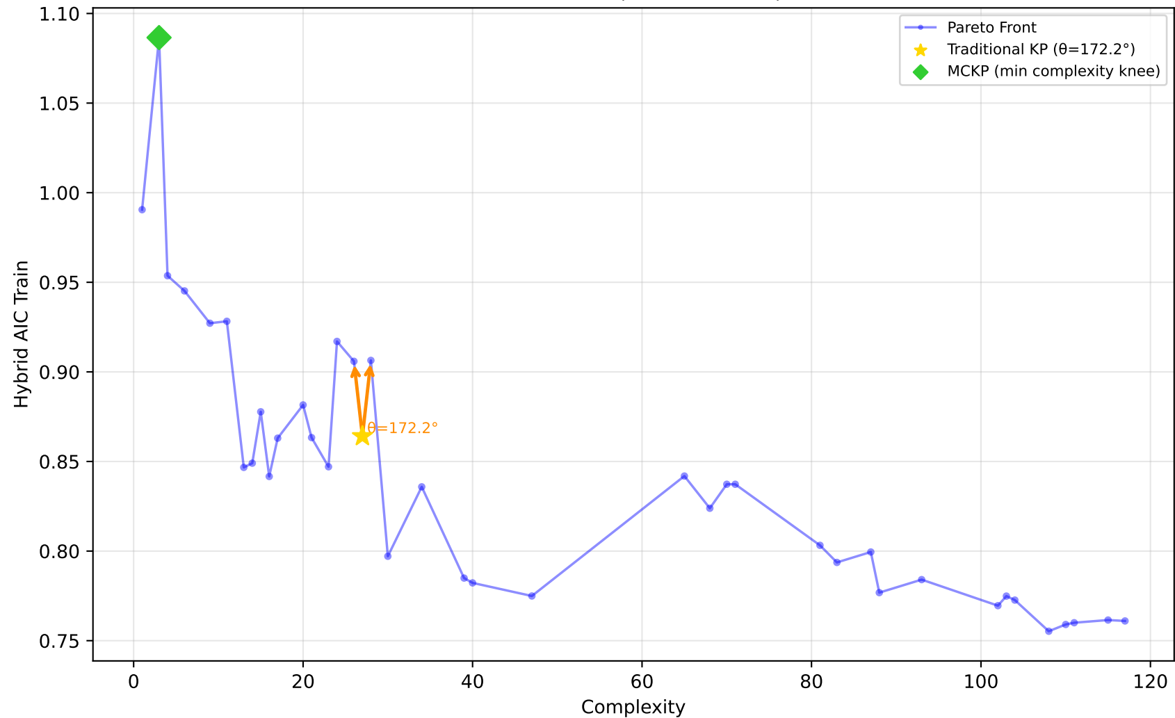
637_fri_c1_500_50 - Run 17 - MVP - Hybrid AIC Train \lambda_1=0.10, \lambda_2=0.00, \lambda_3=1.00 | Difficulty: 1.00 | Method: hmr
