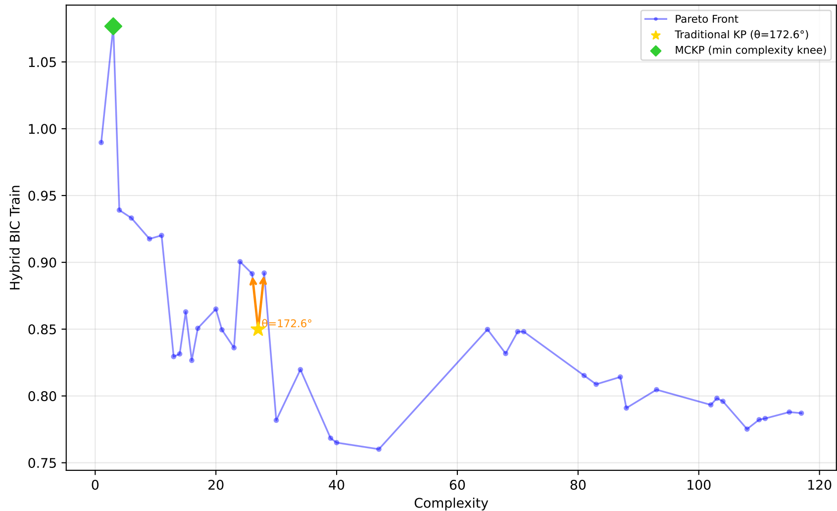
637_fri_c1_500_50 - Run 17 - MVP - Hybrid BIC Train \lambda_1=0.10 , \lambda_2=0.00 , \lambda_3=1.00 | Difficulty: 1.00 | Method: hmr
