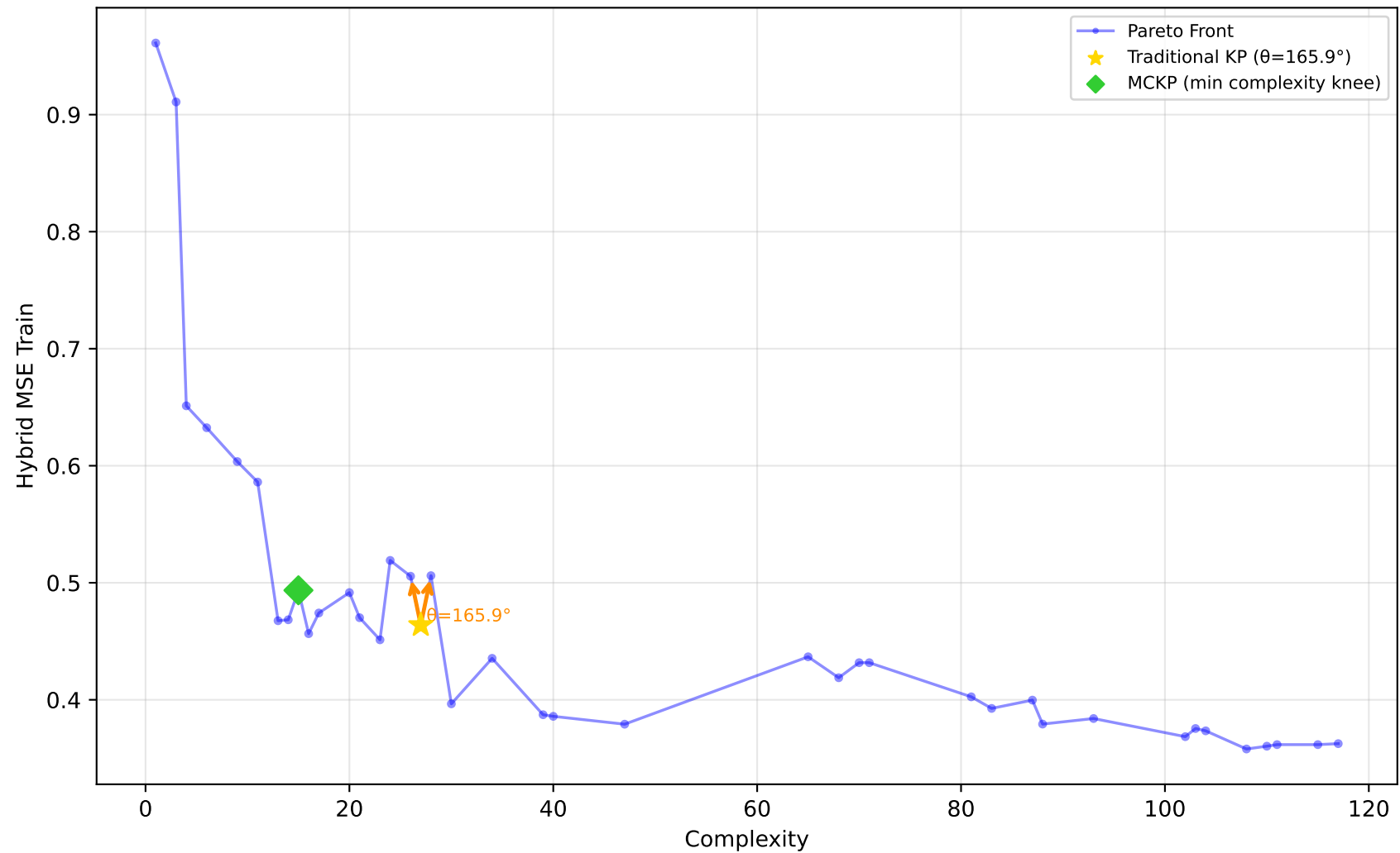
637_fri_c1_500_50 - Run 17 - MVP - Hybrid MSE Train \lambda_1=0.10, \lambda_2=0.00, \lambda_3=1.00 | Difficulty: 1.00 | Method: hmr
