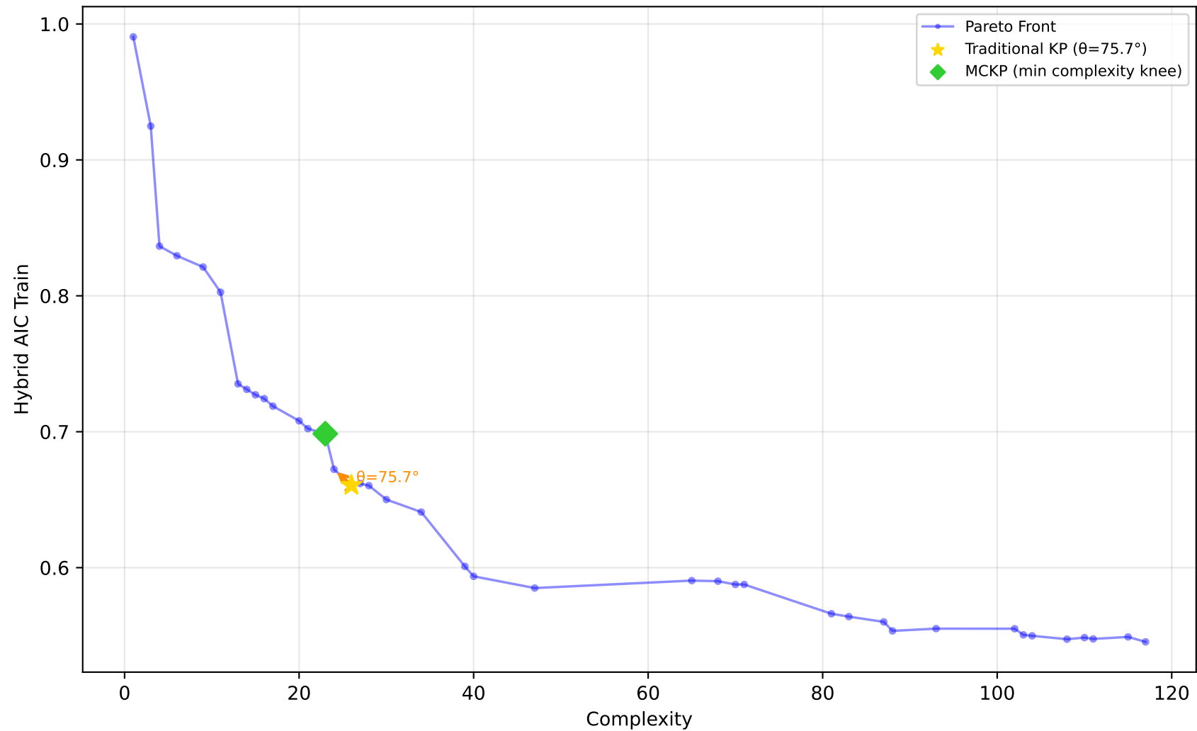
637_fri_c1_500_50 - Run 17 - SVP - Hybrid AIC Train \lambda_1=0.00, \lambda_2=0.00, \lambda_3=0.00 | Difficulty: 1.00 | Method: hmr
