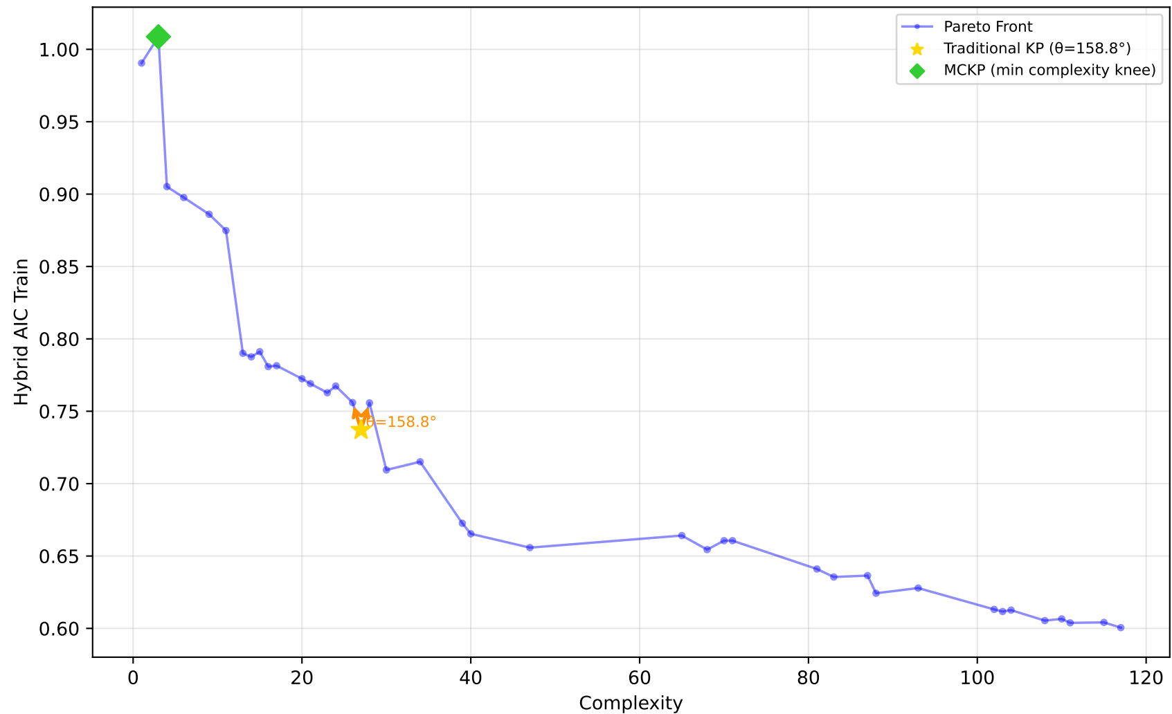
637_fri_c1_500_50 - Run 17 - SVP - Hybrid AIC Train \lambda_1=0.10 , \lambda_2=0.00 , \lambda_3=0.20 | Difficulty: 1.00 | Method: hmr
