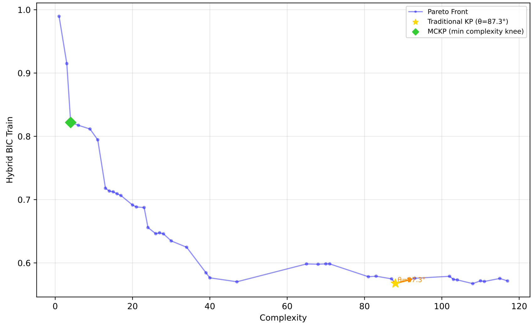
637_fri_c1_500_50 - Run 17 - SVP - Hybrid BIC Train \lambda_1=0.00, \lambda_2=0.00, \lambda_3=0.00 | Difficulty: 1.00 | Method: hmr
