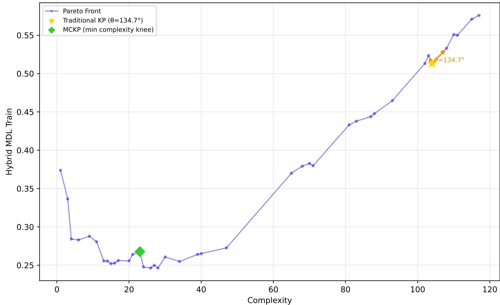
637_fri_c1_500_50 - Run 17 - SVP - Hybrid MDL Train \lambda_1=0.00 , \lambda_2=0.00 , \lambda_3=0.00 | Difficulty: 1.00 | Method: hmr
