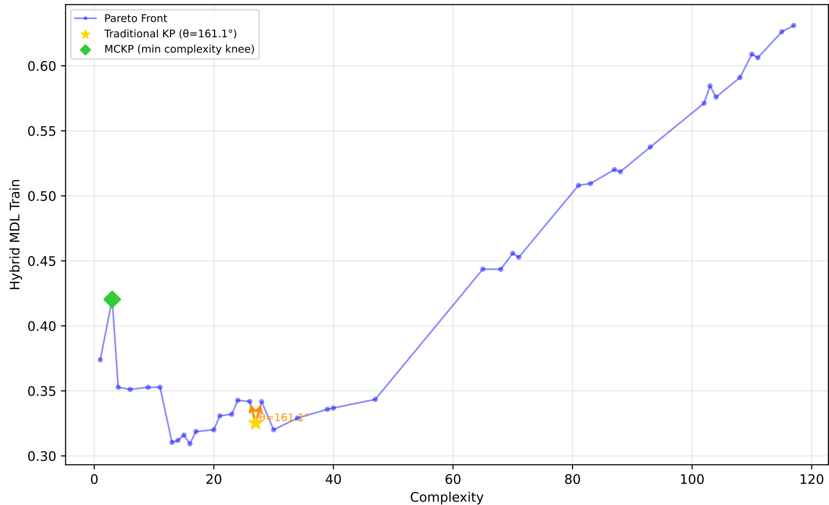
637_fri_c1_500_50 - Run 17 - SVP - Hybrid MDL Train \lambda_1=0.10, \lambda_2=0.00, \lambda_3=0.20 | Difficulty: 1.00 | Method: hmr
