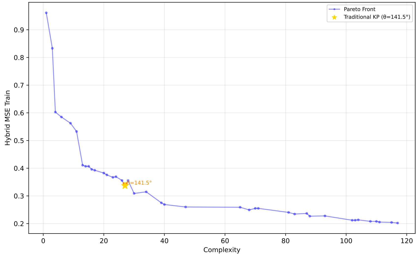
637_fri_c1_500_50 - Run 17 - SVP - Hybrid MSE Train \lambda_1=0.10, \lambda_2=0.00, \lambda_3=0.20 | Difficulty: 1.00 | Method: hmr
