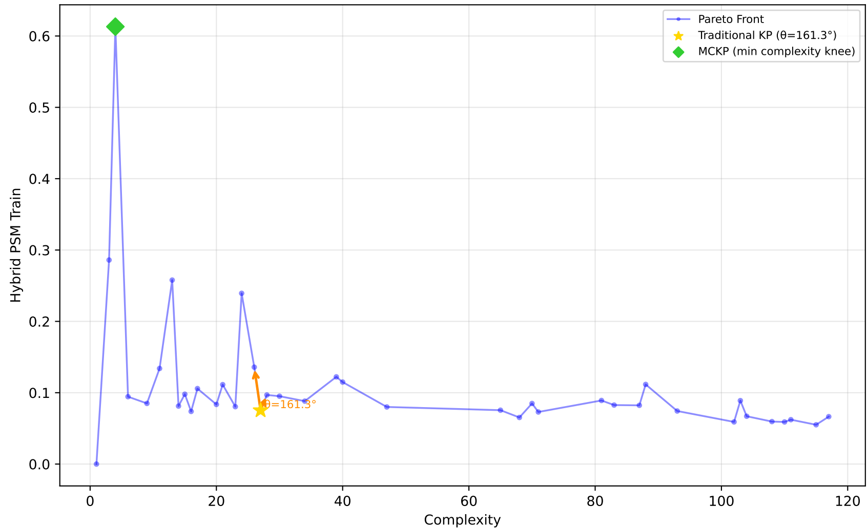
637_fri_c1_500_50 - Run 17 - SVP - Hybrid PSM Train \lambda_1=0.10, \lambda_2=0.00, \lambda_3=0.20 | Difficulty: 1.00 | Method: hmr
