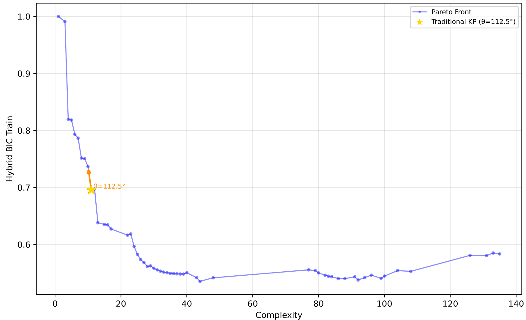
637_fri_c1_500_50 - Run 18 - MVP - Hybrid BIC Train \lambda_1=0.00, \lambda_2=0.50, \lambda_3=0.00 | Difficulty: 1.00 | Method: hmr
