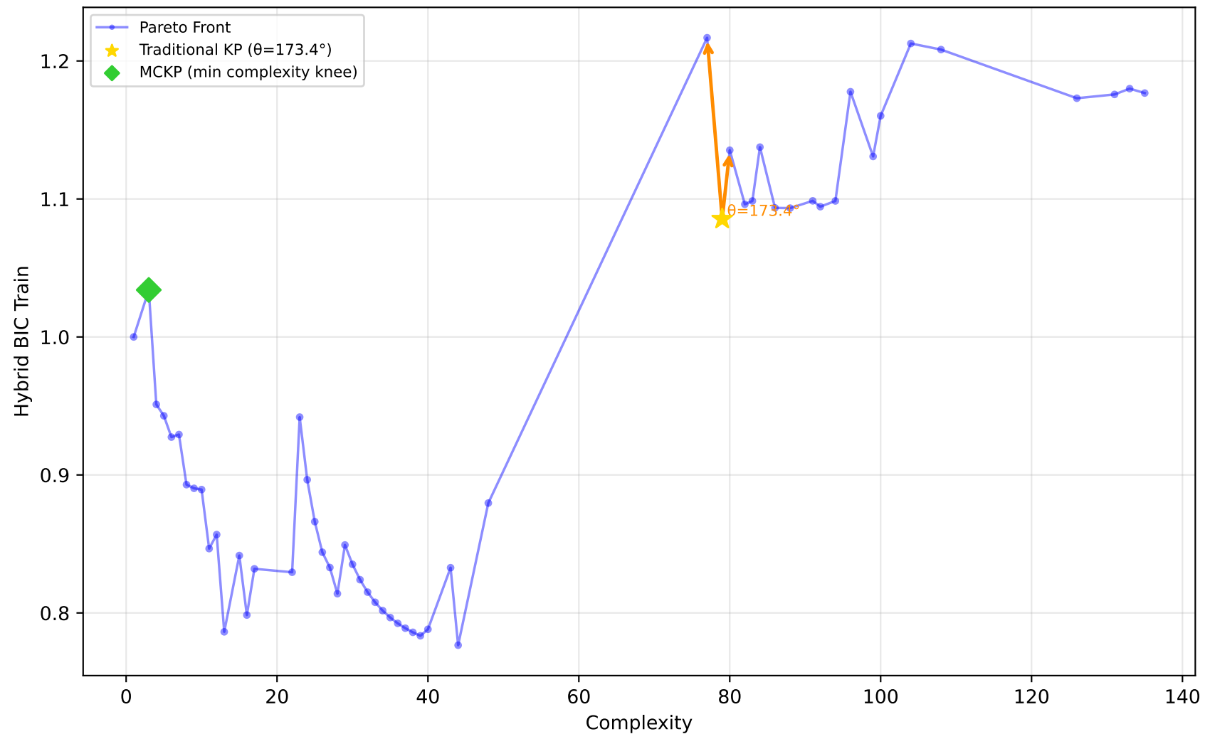
637_fri_c1_500_50 - Run 18 - MVP - Hybrid BIC Train \lambda_1=0.10, \lambda_2=0.00, \lambda_3=1.00 | Difficulty: 1.00 | Method: hmr
