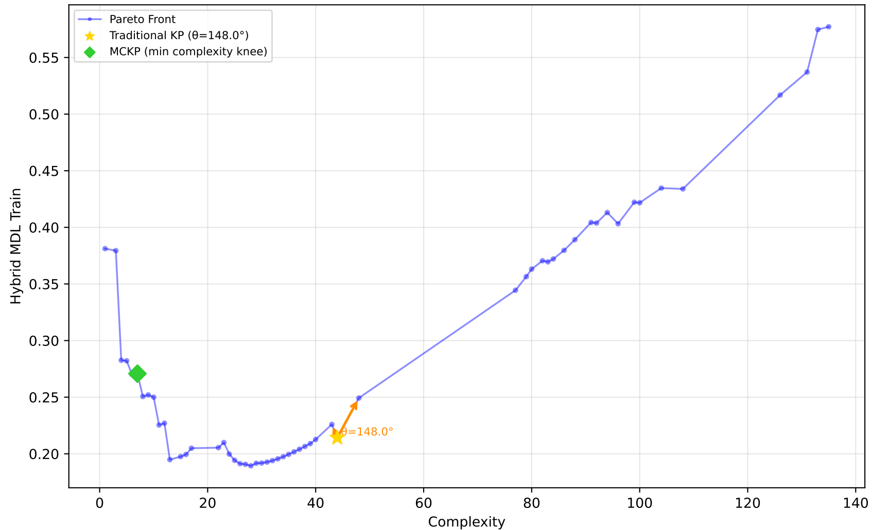
637_fri_c1_500_50 - Run 18 - MVP - Hybrid MDL Train \lambda_1=0.00 , \lambda_2=0.50 , \lambda_3=0.00 | Difficulty: 1.00 | Method: hmr
