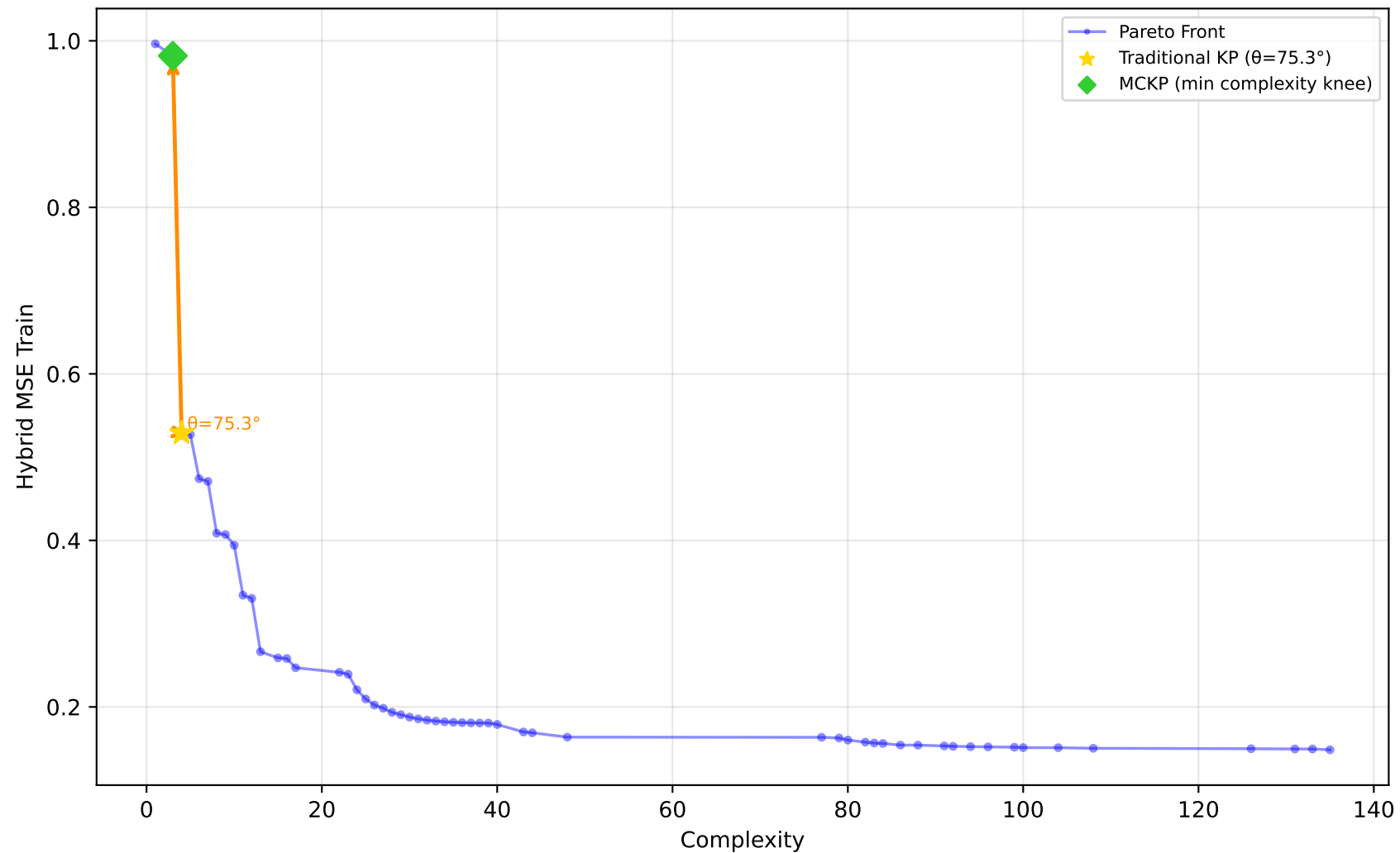
637_fri_c1_500_50 - Run 18 - MVP - Hybrid MSE Train \lambda_1=0.00, \lambda_2=0.50, \lambda_3=0.00 | Difficulty: 1.00 | Method: hmr
