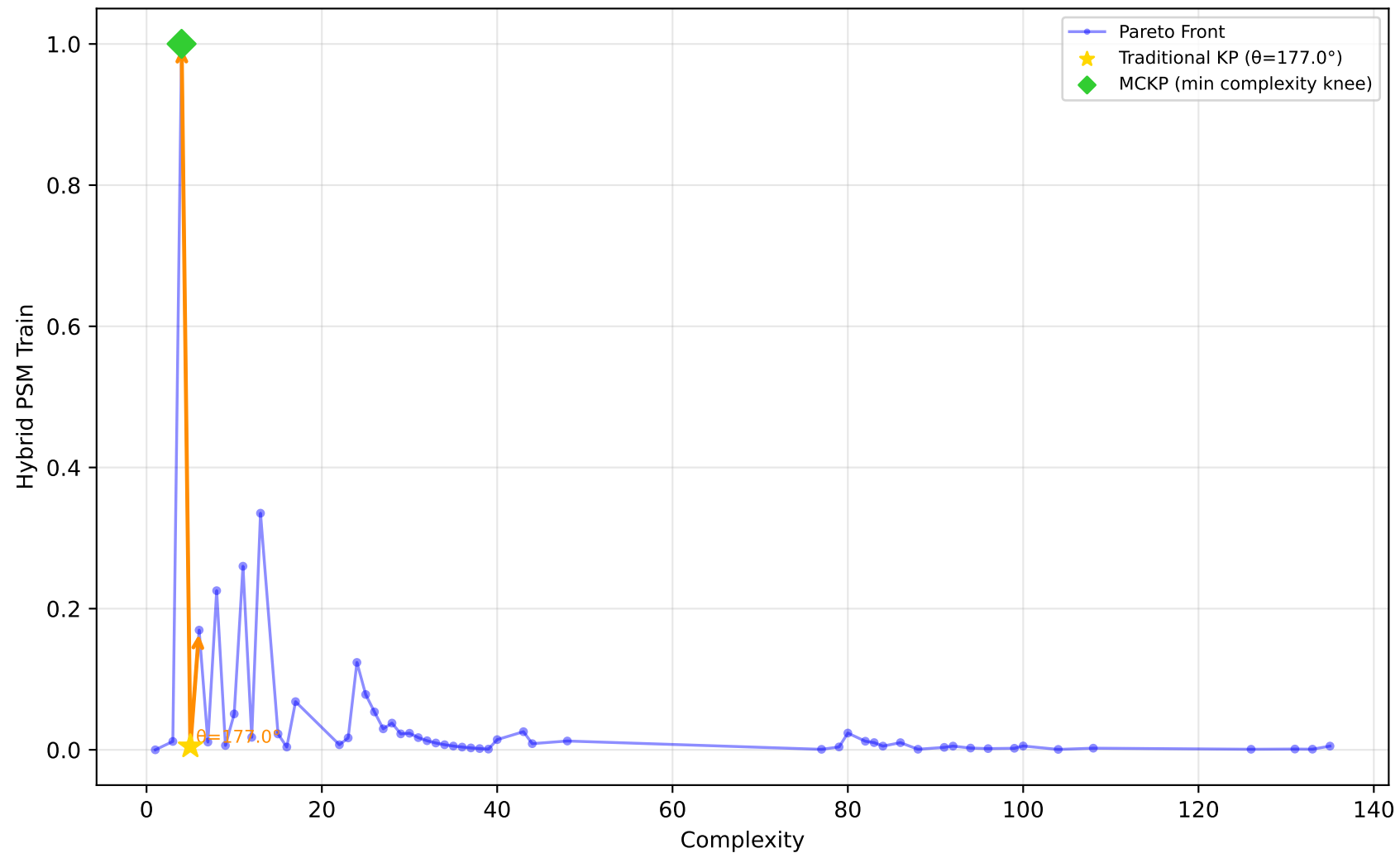
637_fri_c1_500_50 - Run 18 - MVP - Hybrid PSM Train \lambda_1=0.00, \lambda_2=0.50, \lambda_3=0.00 | Difficulty: 1.00 | Method: hmr
