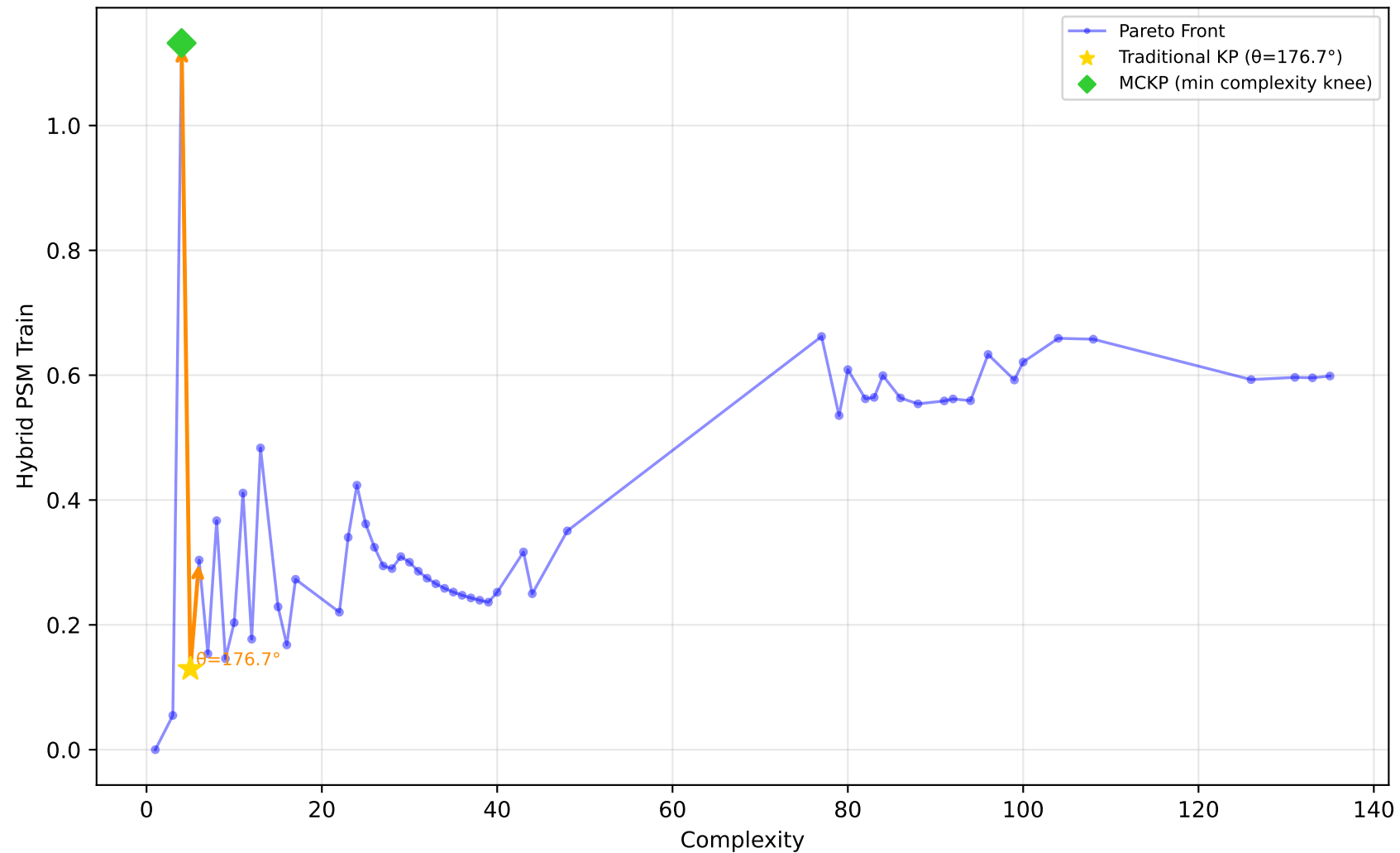
637_fri_c1_500_50 - Run 18 - MVP - Hybrid PSM Train \lambda_1=0.10, \lambda_2=0.00, \lambda_3=1.00 | Difficulty: 1.00 | Method: hmr
